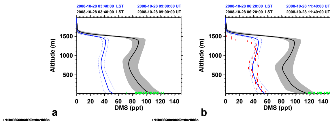
Fig. 10. Comparison of DMS from simulation S_0 (black) and S_1 (blue) at (a) 09:00 UT and (b) 11:40 UT with VOCALS-REx RF06 POC observations at 11:36 UT (red dots) on board the NCAR C-130 aircraft, and surface measurements during a 1 h period centered around the indicated times on board the NOAA research vessel Ronald H. Brown (green bars). Solid curves denote the model mean, gray shading and dotted blue curves model values between the 10th and 90th percentile.
