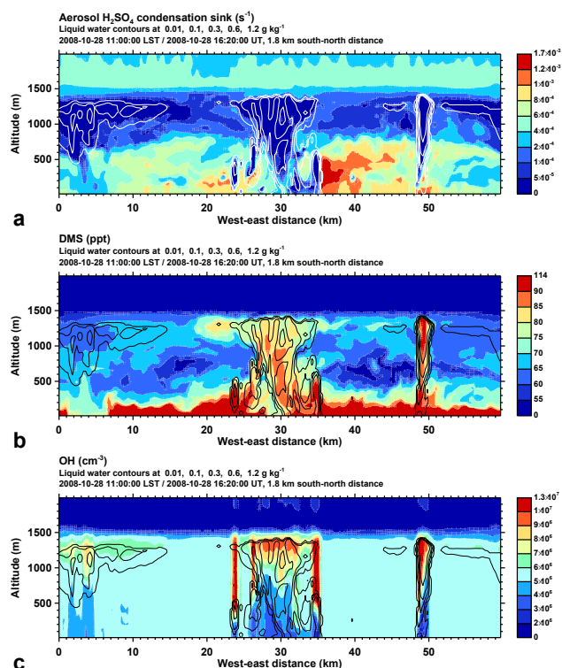
Fig. 4. Vertical slices through the domain of simulation S_0 at 28 October 2008 16:20 UT. Contour lines denote liquid water (sum of cloud and rain water). (a) Cloud processes in open cell updrafts deplete aerosol particles and reduce the aerosol \text{H}_2\text{SO}_4 condensation sink, which is lowest inside clouds. The clean, cloud-processed air detrains in the upper boundary layer and forms an ultra-clean layer with low aerosol \text{H}_2\text{SO}_4 condensation sink values. (b) Updrafts lift DMS emitted from the ocean into the upper boundary layer. (c) Scattering of solar radiation around cloud tops results in elevated OH concentrations, which oxidize DMS to \text{SO}_2 .
