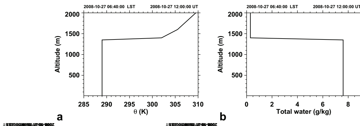
Fig. 1. Initial vertical profile of (a) potential temperature and (b) total water mixing ratio, present as water vapor at the start of the simulations.
