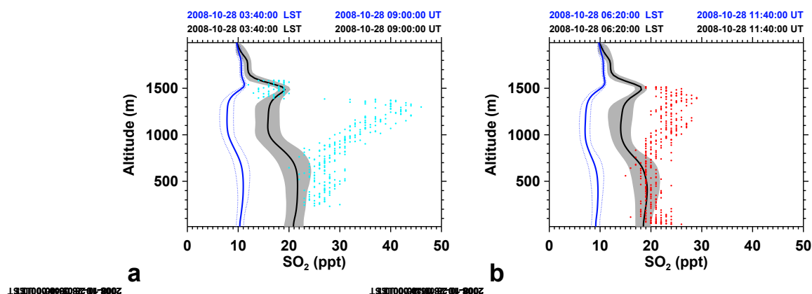
Fig. 11. Comparison of \text{SO}_2 from simulation S_0 (black) and S_1 (blue) at (a) 09:00 UT and (b) 11:40 UT with VOCALS-REx RF06 POC observations at 09:05 UT (cyan dots) and at 11:36 UT (red dots) on board the NCAR C-130 aircraft. Solid curves denote the model mean, gray shading and dotted blue curves model values between the 10th and 90th percentile.
