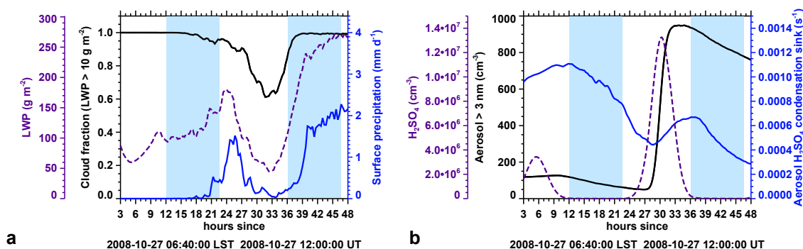
Fig. 3. Time series from simulation S_0 of (a) domain-averaged liquid water path, cloud fraction, and precipitation, and of (b) gas phase sulfuric acid concentration, concentration of aerosol particles larger than 3 nm in dry diameter, and aerosol sulfuric acid condensation sink, averaged over cloud-free locations in the boundary layer. Light blue shading indicates nighttime.
