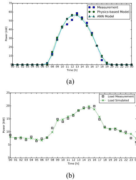
Figure 5(a) Comparison of the simulated PV power with the measurements (b) Comparison of the total predicted and real power of the energy loads in HGV. Both are on August 25, 2014
