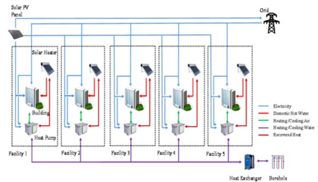
Figure 2 The schematic of the energy systems of HGV
