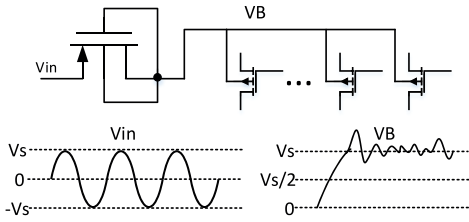
Fig. 5. Peak detector for WP-ECRL and CEPAL.
