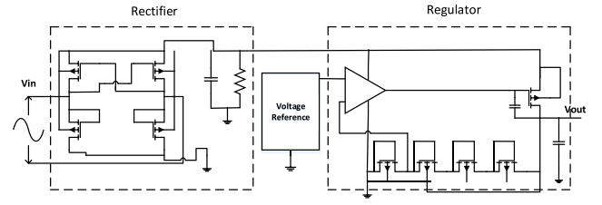
Fig. 7. Rectifier and regulator required for the conventional approach.
