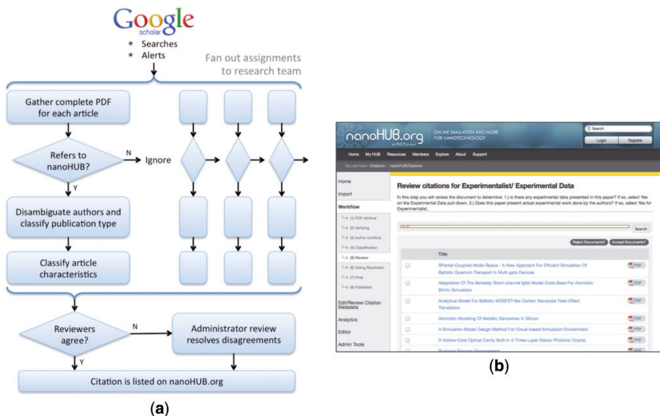
Figure 3. (a) The process of gathering citations related to nanoHUB.org, and (b) the web infrastructure that supports that process.
