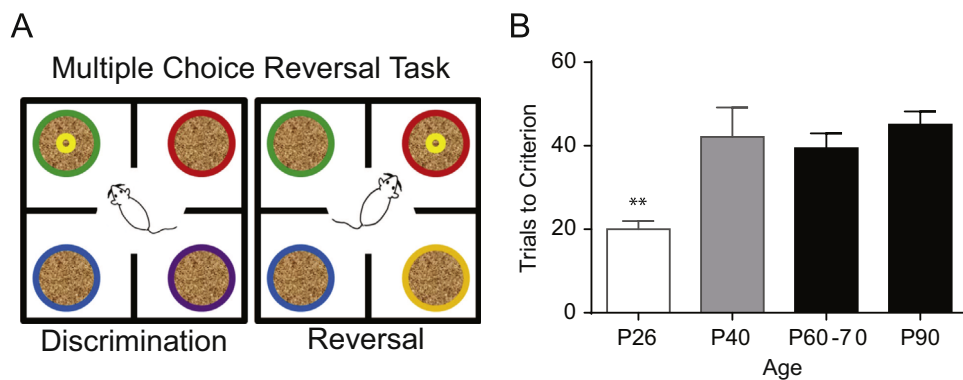
Fig. 4. Age-dependent changes in behavioral flexibility in a multiple choice reversal task. A) A schematic of the task used in our lab (Johnson and Wilbrecht, 2011). Each color represents an odor. Mice are released from a central cylinder to start a trial. In the discrimination phase mice must learn to dig in the correct odor to receive a food reward. After the mouse completes 8 out of 10 correct trials the reversal phase begins in which a previously unpaired scent predicts the food reward. B) Prepubertal (P26) mice make significantly fewer reversal errors ( F_{3,96}=12.00 ; p < 0.01 ) than mid-adolescent mice (P40) or adult mice (P60–90).
