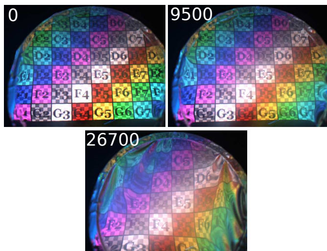
Fig. 9. Photographs showing the result of our deformation test to estimate usability over lifetime for our in-house built deformable membrane mirror. We iterate on stretching the deformable membrane mirror back and forth with 10 times larger deformations than we use during operation. Each photograph shows a counter that represents number of iterations.
