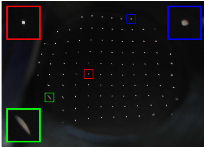
Fig. 12. A view approximating the point spread function across the membrane. Squares of 3x3 pixels are illuminated in a grid pattern to show the graceful degradation of focus across the membrane. Central region shows minimal point spread (red inset), while periphery shows a much larger point spread (blue inset). Severe defocus in lower left region (green inset) is caused by inadequate tension on membrane when closing and securing the housing.
