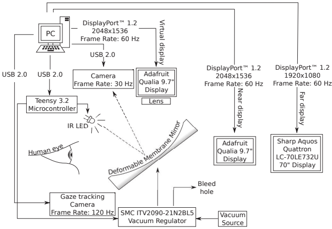
Fig. 7. A sketch showing the system overview and connections of the hardware in our prototype.
