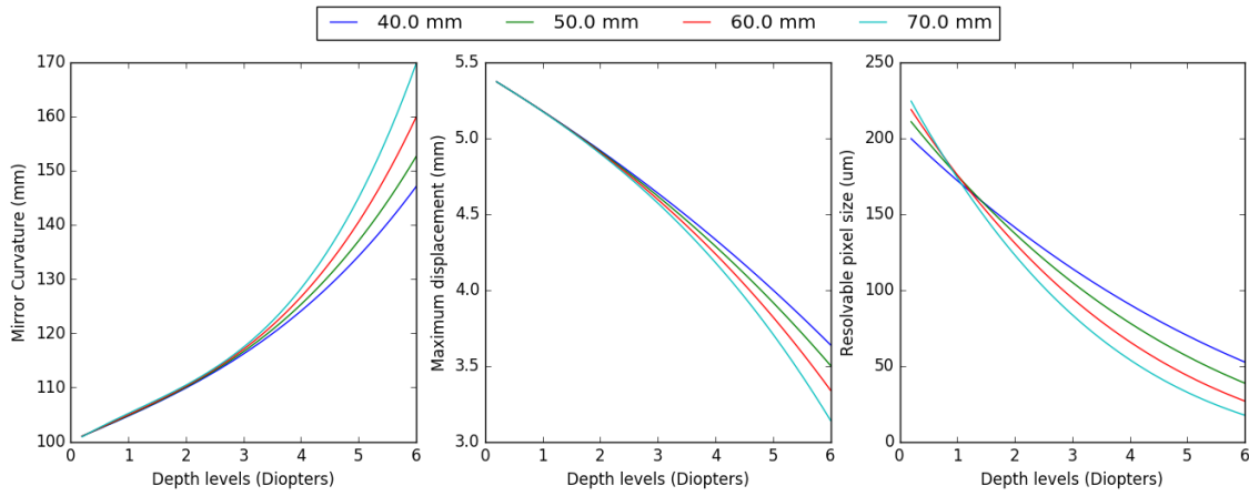
Fig. 4. A sample design is evaluated for different eye reliefs d_{eye\ relief} with a configuration of an aperture size d_{aperture} = 50 mm in horizontal axis, an aperture size d_{aperture} = 65 mm in vertical axis, a mirror tilt \beta = 45^\circ , a screen tilt \alpha = 20^\circ , an eye box d_{eye\ box} = 20 mm, and a screen distance d_{display} = 60 mm. For all evaluations, on-axis depth fields as shown in Figure 2 are chosen at different depth levels. A deformable membrane mirror's curvature is calculated for different depth levels as shown on the left. The maximum amount of displacement required by each depth level is shown in the middle figure. Assuming an eye with an aperture size of 6 mm, resolvable pixel size on a screen inside the given eye box is calculated for different depth levels as shown in the figure on the right. Smaller d_{eye\ relief} benefits the design by decreasing required displacement on a membrane, however resolution improves at closer depths with a larger d_{eye\ relief} .
