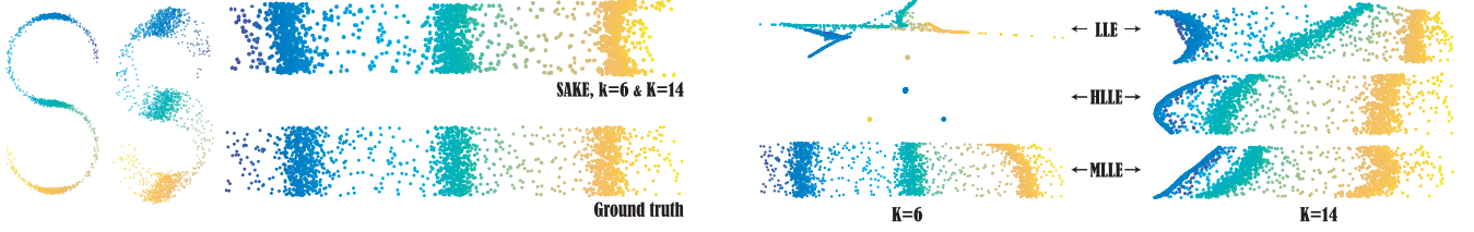
Figure 10: S-shaped manifold with variable density and Gaussian noise. SAKE is also robust to variable density in the input. A non-uniformly sampled ‘S’ shape is embedded in 3D with Gaussian noise added (left, profile views). We compare our results with other existing approaches, for various parameters.
