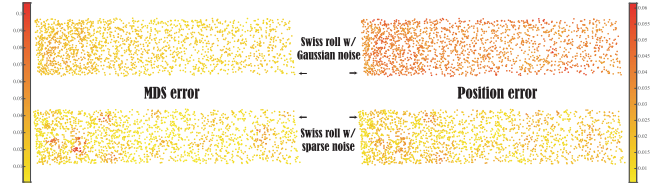
Figure 9: Embedding errors. For the SAKE results shown in Fig. 8 (top) and Fig. 7 (bottom), we show the local reconstruction errors in pairwise distances (MDS errors, left) and in relative l^2 position errors (right).
