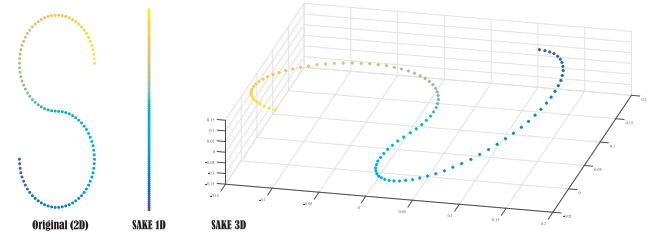
Figure 15: Choice of dimensionality. For a 2D S-shaped pointset (left), its reduction to 1D provides the expected parameterization (middle); a 2D embedding would return the exact same input shape as the original; a 3D embedding, instead, exhibits unexpected distortions in the extra dimension (right); and of course, a 0D embedding would lose injectivity.
