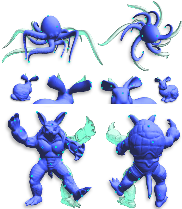
Figure 14: Zoo. We use our SAKE editing approach on a few basic 3D models. Light blue markers indicate handle vertices (held fixed or displaced). All models use the same editing parameters; a subsampled medial axis was only added to the octopus model (20 added points) to increase the volume rigidity of the long and thin tentacles.
