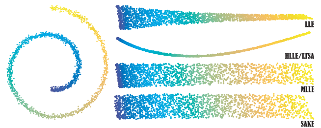
Figure 8: Swiss roll with Gaussian noise. SAKE can handle strong noise in the input. Here, points are sampled from a 2D Swiss roll embedded in 3D with added Gaussian noise along the normal (left, profile view). Results of 2D embeddings (right, top to bottom): LLE ( k = 15 ), HLLS/LTSA ( k = 15 ), MLLE ( k = 15 ) and SAKE ( k = 15, K = 75 ). Again, LTSA and HLLS return visually identical results, significantly deformed due to the instability of PCA-based tangent plane approximation in presence of strong noise.
