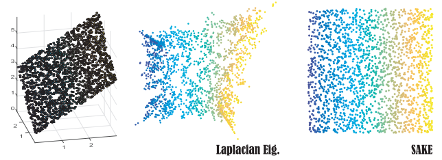
Figure 2: Affine Precision. Laplacian Eigenmap (middle) is not linearly precise as it fails to properly capture a uniformly sampled flat patch in 3D (left). SAKE (right) does not suffer from this common limitation.
