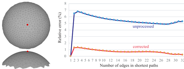
Figure 4: Geodesic distance correction. From a triangulated patch of a spherical cap with good aspect ratio elements (left, top and side views), the total relative L^2 error of all pairwise distances computed based on Dijkstra’s shortest paths is 29.9; our simple post-processing reduces the error to 6.5. If we bin all the distances based on the number of edges in the edge-based connecting paths, we see that aside from the case of a single edge (where the geodesic distance cannot be improved), our geodesic distance correction reduces errors by a factor five or more.
