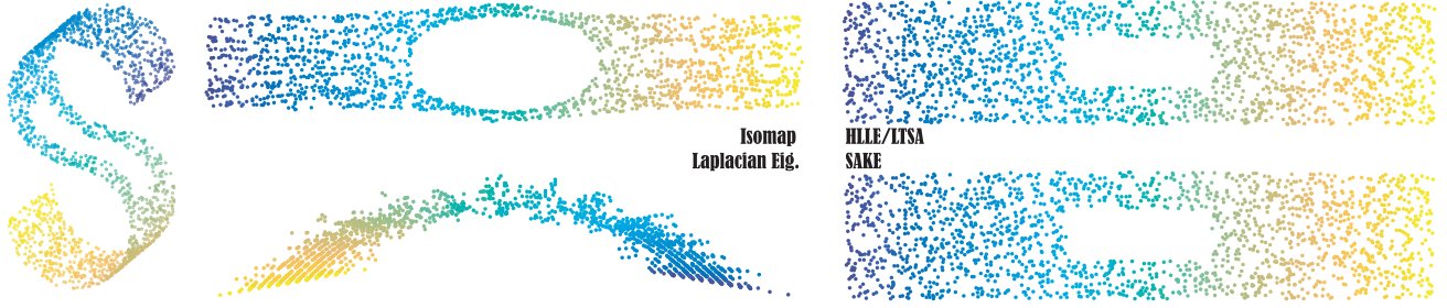
Figure 3: Non-simply connected manifold. For points uniformly distributed over a 2-dimensional S-shaped manifold containing a hole (left), Isomap (top middle) overestimates the size of the hole, while Laplacian Eigenmaps result (bottom middle) is severely distorted. However, HLL with k=12 (top right) and Sake with k=K=12 (bottom right) recover close to perfect embeddings in this noiseless case.
