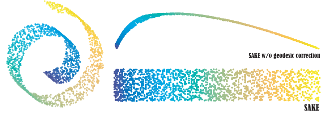
Figure 5: Geodesic curvature correction. Our geometric correction improves geodesic approximations for coarse and irregularly sampled data; without it, extreme distortion can happen on imperfectly sampled datasets. We set k = K = 12 for this noiseless Swiss Roll example (left).
