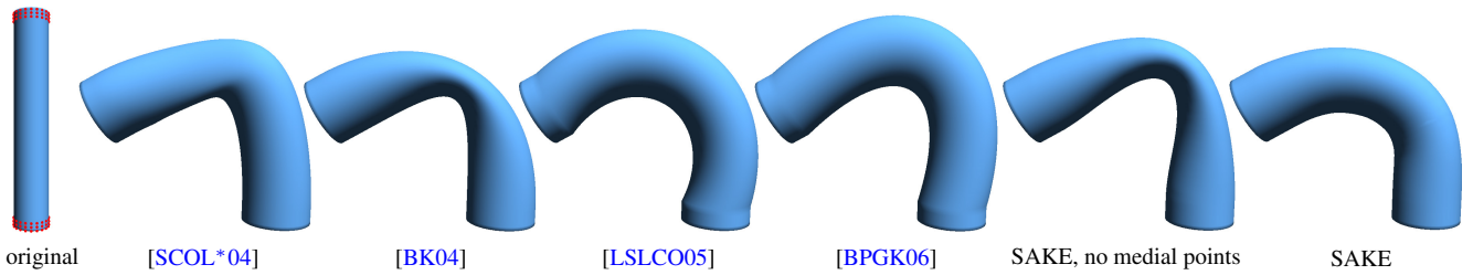
Figure 13: Bending bars. We compare our approach (with and without added medial points for clarity) with a number of existing deformation methods on the 120° bend example with handles (marked in red on the original mesh) taken from [BS08]. Note the absence of artifacts near the pinned extremities for SAKE.
