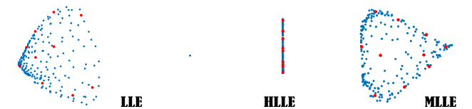
Figure 12: Knights. Examples of results for the knights images (see Fig. 1 for comparison). Other methods give markedly more distorted results; HLLE, in particular, fails to return a valid parameterization.
