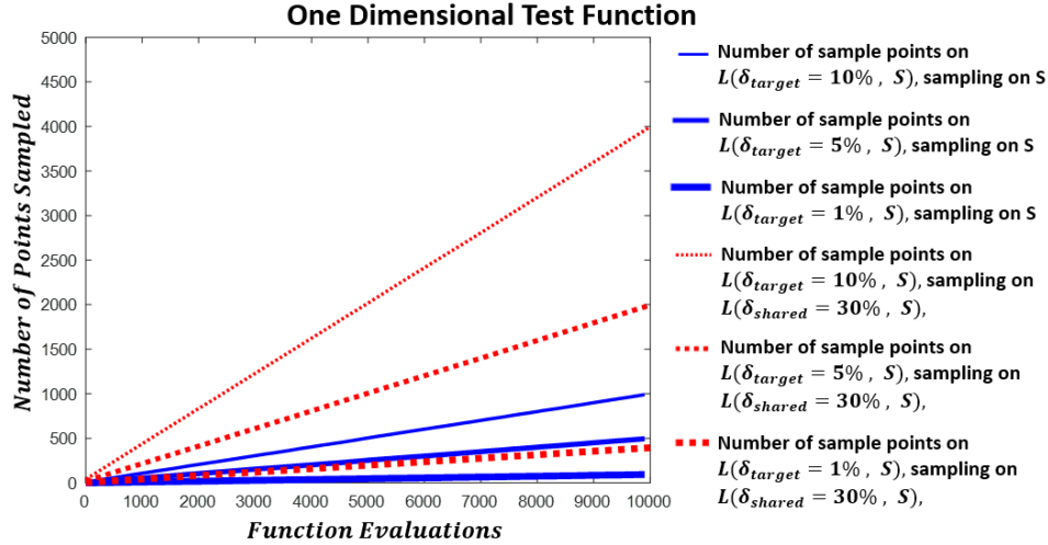
Figure 2: Number of sample points within target quantiles ( \delta_{\text{target}} = 10\%, 5\%, 1\% ) from either the level set approximation \tilde{\Sigma}_k with \delta_{\text{shared}} = 0.3 (broken line), or random sampling on the entire domain S (solid line) for the one-dimensional test function in (7). The vertical axis shows the number of points sampled, averaged across 30 experiments. The horizontal axis tracks the number of high-fidelity function evaluations.
