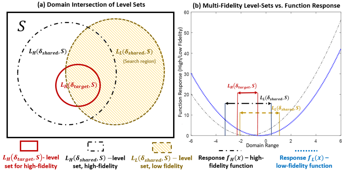
Figure 1: A graph of intersecting level sets between a high-fidelity function and a low-fidelity function on a common domain. In (a), L_L(\delta_{\text{shared}}, S) is outlined with a dashed line, L_H(\delta_{\text{shared}}, S) is outlined with a dash-dot line, and L_H(\delta_{\text{target}}, S) is outlined with a solid line. In (b), the level sets are shown relative to their function responses.
