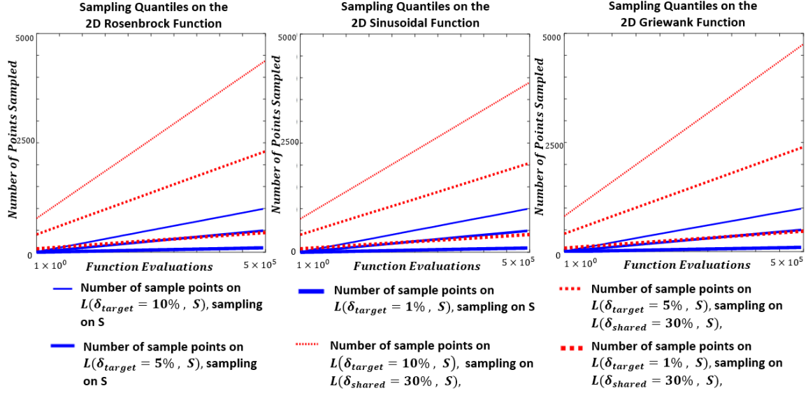
Figure 4: Number of sampled points within target quantiles ( \delta_{\text{target}} = 10\%, 5\%, 1\% ) from either the level set approximation \tilde{\Sigma}_k generated by the PBnB algorithm with \delta_{\text{shared}} = 0.3 (broken line), or random sampling on the entire domain S (solid line) for the Rosenbrock, Sinusoidal, and Griewank Functions. The vertical axis shows the number of points sampled, averaged across 30 experiments. The horizontal axis tracks the number of high-fidelity function evaluations.
