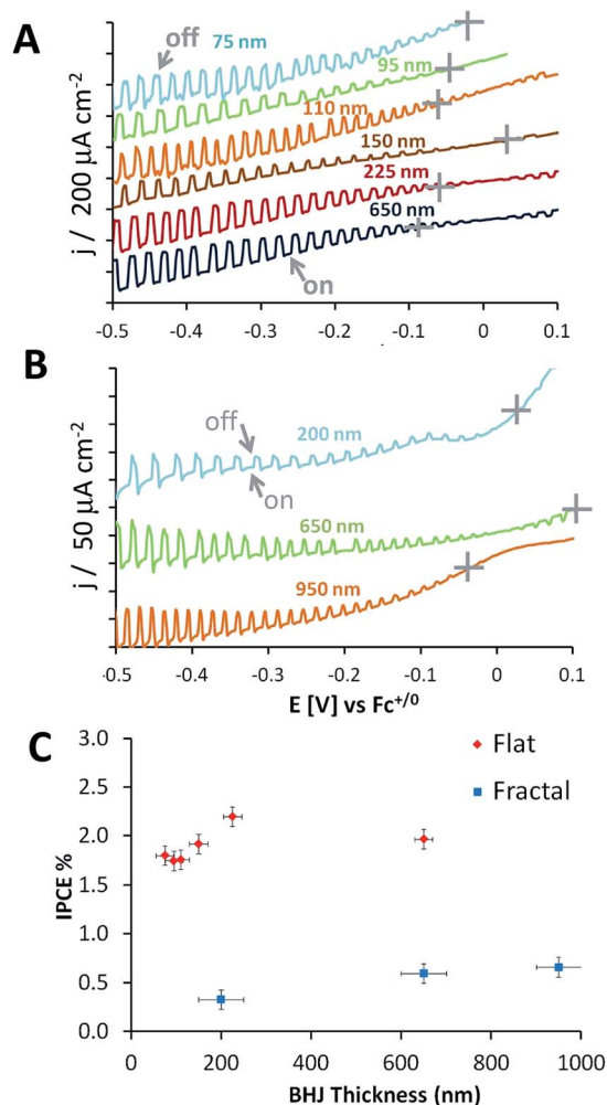
Fig. 8 Photoelectrochemical data for BHJ/PEDOT:PSS films on (A) flat and (B) fractal silver electrodes, as a function of BHJ thickness. Conditions: 0.01 M ( \text{Bu}_4\text{N})\text{PF}_6 , 0.005 M \text{FcBF}_4 in \text{CH}_3\text{CN} using 435 nm LED ( 10\text{--}20 \text{ mW cm}^{-2} ). Potentials are reported versus the \text{Fc}^{+/0} potential of +0.4 V (vs. NHE). Cross-bars indicate zero current. (C) Incident photon to current efficiencies (IPCE%) versus active layer thickness.
