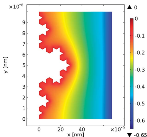
Fig. 1 Computed electric potential (color bar in volts) in a P3HT:PCBM film adjacent to a metallic Koch fractal electrode (enclosed white area). The length of the fractal perimeter is 237 nm. The thickness of the polymer film device is 68 nm. It is illuminated from the right side. The model (see ref. 33) is solved using a finite-element method (COMSOL), and takes into account charge generation, recombination (both Langvin and Shockley–Reed–Hall), transport, and diffusion.
