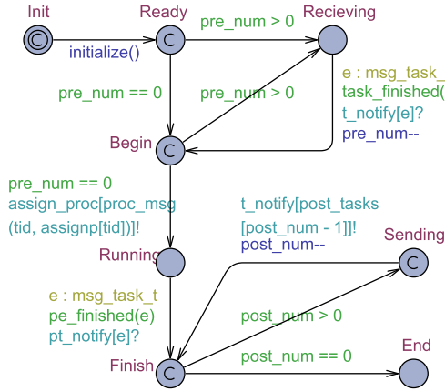
Fig. 4. Front-end model of a task
