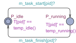
Fig. 7. Front-end model of the temperature monitor
