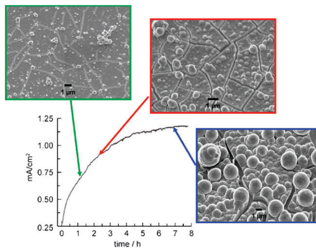
Fig. 1 Current density profile for bulk electrolysis at 1.29 V (vs. NHE) in 0.1 M KPi electrolyte at pH 7.0 containing 0.5 mM \text{Co}^{2+} . SEM images of the electrode surface taken at indicated time points during the electrodeposition of the catalyst film. The ITO substrate can be seen through cracks in the dried film.
