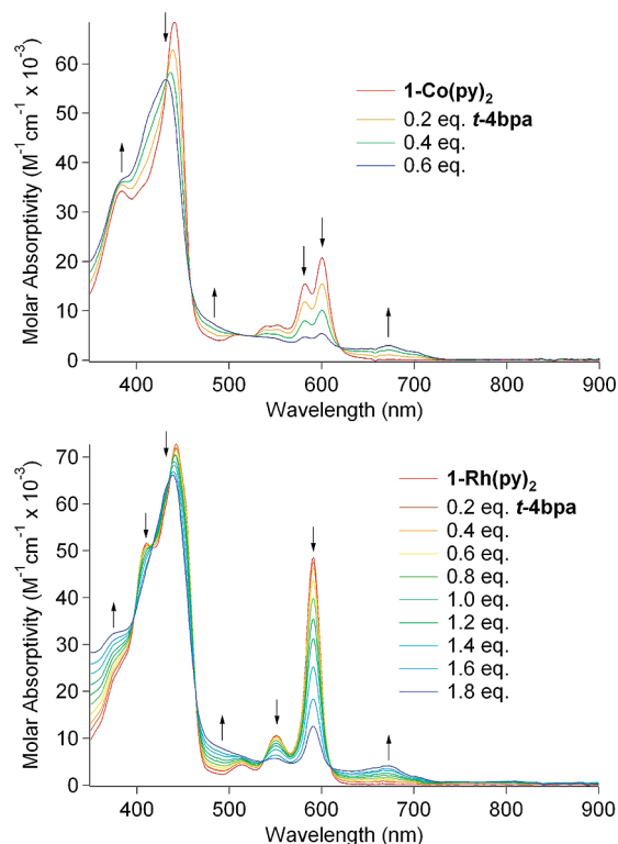
Figure 9. Absorption spectral changes accompanying oxidation of 1-Co(py) 2 (top) and 1-Rh(py) 2 (bottom) by t-4bpa in CH 2 Cl 2 solutions. Reaction with the Co(III) complex was terminated after addition of 0.6 equiv, owing to product instability. 26b
