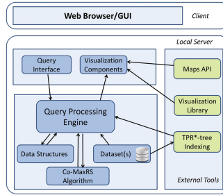
Fig. 2. Software architecture.
