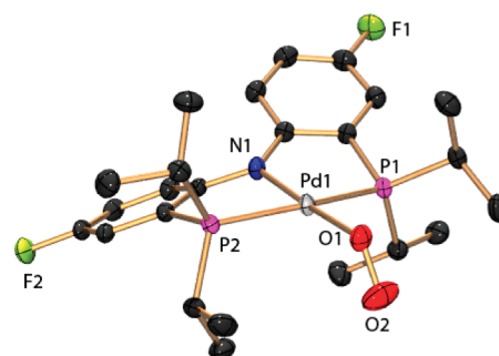
Figure 2. POV-Ray 17 rendition of the ORTEP 18 drawing (50% thermal ellipsoids) of (\text{FPNP})\text{PdO}_2 showing selected atom labeling. Hydrogen atoms and the THF solvent molecule have been omitted for clarity. Selected bond distances (Å) and angles (deg): Pd1–P1, 2.2886(5); Pd1–P2, 2.2981(4); Pd1–O1, 2.0096(13); Pd1–N1, 2.0263(14); O1–O2, 1.293(2); P1–Pd1–P2, 165.129(17); O1–Pd1–N1, 176.49(6); Pd1–O1–O2, 113.79(12).
