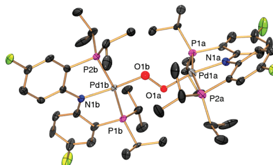
Figure 3. POV-Ray 17 rendition of the ORTEP 18 drawing (50% thermal ellipsoids) of [(\text{FPNP})\text{PdO}]_2 showing selected atom labeling. Hydrogen atoms and the isopropyl Me groups have been omitted for clarity. Selected bond distances (Å) and angles (deg): O1a–O1b, 1.47(2); N1a–Pd1a, 2.032(8); O1a–Pd1a, 1.985(13); O1b–Pd1b, 2.046(14); P1a–Pd1a, 2.290(3); P2a–Pd1a, 2.288(3); O1a–Pd1a–N1a, 163.7(5); P2a–Pd1a–P1a, 166.51(11); O1b–Pd1b–N1b, 167.3(5).
