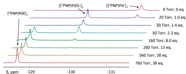
Figure 1. ^{19}\text{F} NMR spectra of the reactions of [(\text{FPNP})\text{Pd}]_2 with different amounts of \text{O}_2 in \text{C}_6\text{D}_6 collected after 5 min in direct sunlight.
