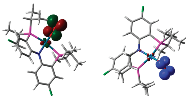
Figure 4. Calculated representation of (left) the singly occupied molecular orbital and (right) the spin density distribution in (^{\text{F}}\text{PNP})\text{PdO}_2 .
