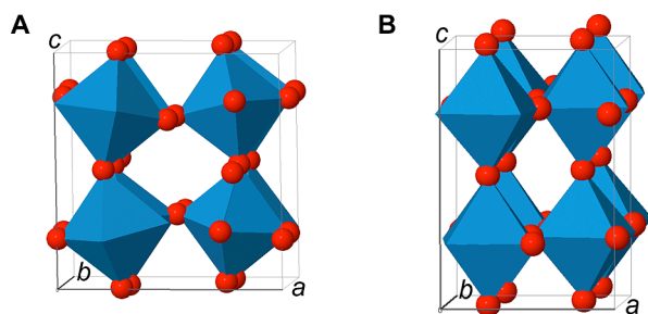
Figure 1. Unit cells of (A) monoclinic \gamma - \text{WO}_3 at room temperature 16 and (B) tetragonal \text{WO}_3 at 800 °C. 17 W atoms are located inside the blue octahedra, and O atoms are represented by red spheres. The void spaces can accommodate small cations and molecules.
