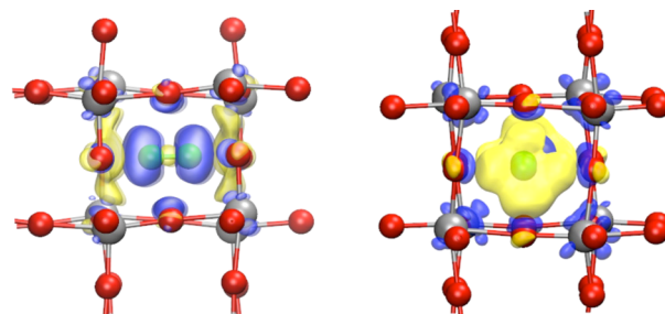
Figure 3. Isosurface of electron density difference for monoclinic \text{WO}_3 with and without \text{N}_2 , viewed from two perspectives: yellow, electron loss; blue, electron gain. Atoms: silver, W; red, O; green, N.
