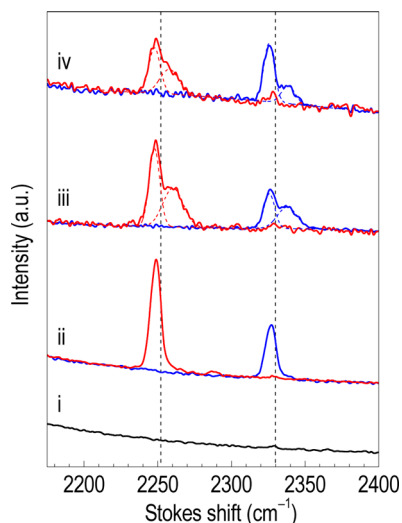
Figure 2. Room-temperature Raman spectra of (i) pure monoclinic \text{WO}_3 , (ii) 0.034\text{N}_2\cdot\text{WO}_3 annealed at 750 °C, (iii) 0.039\text{N}_2\cdot\text{WO}_3 annealed at 550 °C, and (iv) 0.039\text{N}_2\cdot\text{WO}_3 annealed at 420 °C. The solid red and blue curves indicate samples with and without ^{15}\text{N} labeling, respectively. The two dashed vertical lines denote the Stokes shifts of (left) ^{15}\text{N}_2(\text{g}) and (right) ^{14}\text{N}_2 . The dashed red and blue curves show the deconvolution of the observed signal into two Gaussian peaks. a.u. = arbitrary units.
