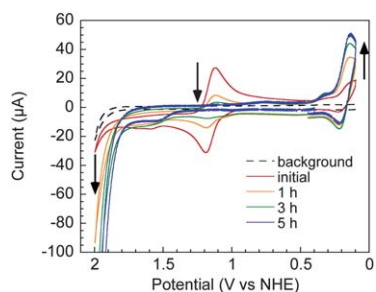
Fig. 1 CVs of [(tpy)(bpy)Co III ] 2 (μ-O 2 )](PF 6 ) 4 ( 1 ) (0.25 mM) in 0.1 M pH 2.1 phosphate.
