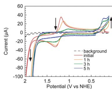
Fig. 2 CVs of the hydroxo-peroxo-bridged (bpy) 2 Co III dimer 2 (0.25 mM) in 0.1 M pH 2.1 phosphate.
