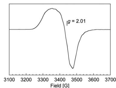
Fig. 5 X-band EPR spectrum of one-electron oxidized 5 ( 0.5 \text{ mM} ) in frozen aqueous pH 1 triflic acid at 5 \text{ K} .
