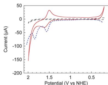
Fig. 4 CVs of FTO background (black dashed), and 5 ( 0.25 \text{ mM} ) in 0.1 \text{ M} pH 2.1 phosphate (red solid) and a differential pulse voltammogram of 5 ( 0.5 \text{ mM} ) using a glassy carbon working electrode (blue dashed), amplitude = 50 \text{ mV} , pulse period = 0.3 \text{ seconds} , vertical axis expanded four-fold for clarity.
