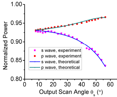
Fig. 6 Power transmission of the output scan beam
