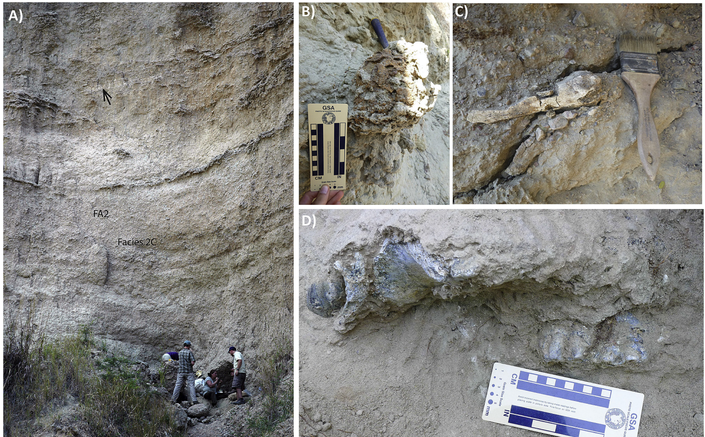
Fig. 6. A) Photograph of a fossil-bearing, sand dominated fluvial channel deposits (FA2: Facies 2C) from the Hamposia section. B–D) Close-up images of termite nest trace fossil (B), mammal fossils (C–D). Note an arrow in Fig. 6A pointing to a volcanic tuff bed (Hippo Tuff) dated at 3.54 \pm 0.13 Ma (Hilbert-Wolf et al., in press).
