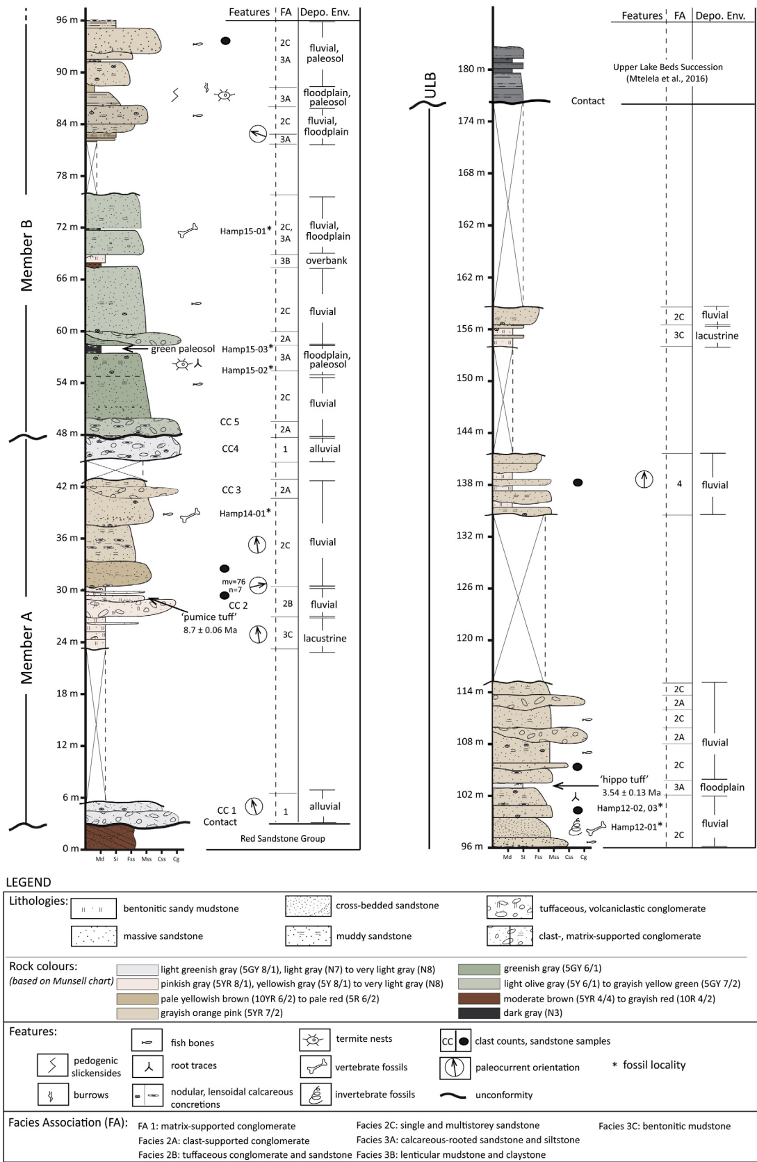
Fig. 3. Lower Lake Beds stratigraphic section measured along the Hamposia River drainage, from 8°37'54"S, 32°49'10"E to 8°34'35"S, 32°49'49"E. U-Pb age data for the Pumice Tuff and Hippo Tuff beds are from Hilbert-Wolf et al. (in press).
