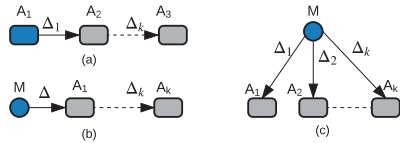
Figure 4: (a) A line of two or more datafiles; (b) A line when the materialized datafile M is not a part of query input; (c) A star.
