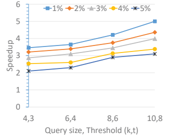
Figure 13: t-Thres. – Effect of |\Delta|
