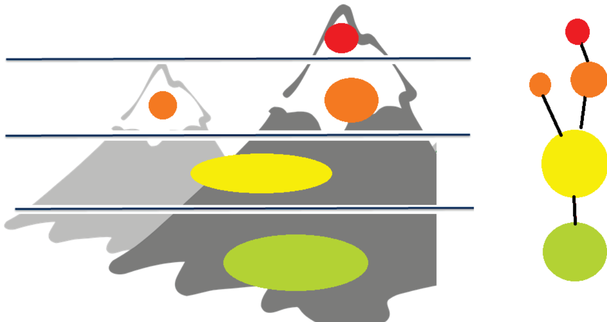
Figure 1: Schematic representation of the illustrative example of use Topological Data Analysis. Here elevation profiles of mountains are examine to understand the different tree populations found in different elevation zones.
