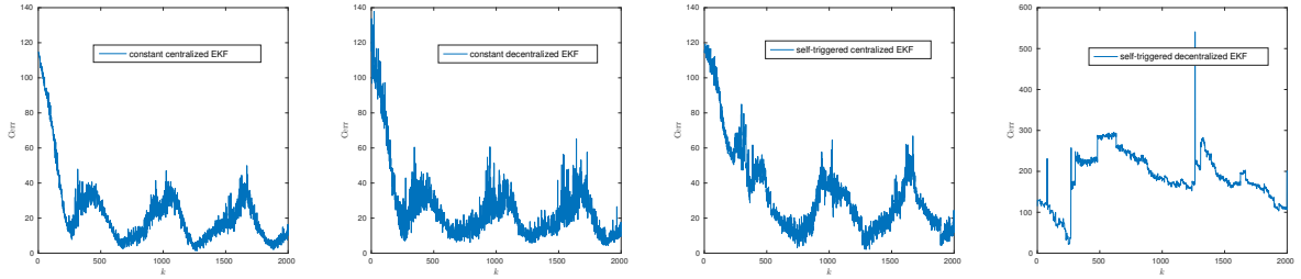
Fig. 7. Convergence error for mobile target tracking with centralized and decentralized EKF estimators steered by the constant strategy and self-triggered strategy
