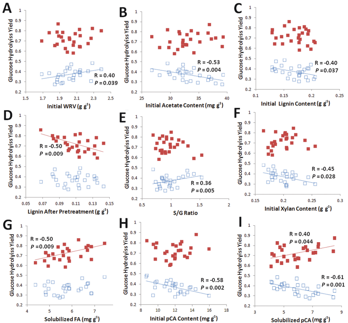
Fig. 4. Summary of significant property correlations with glucose hydrolysis yields. Open data points represent 6 h hydrolysis yields for untreated biomass; filled data points represent 72 h hydrolysis yields for NaOH-pre-treated biomass. Each data point represents the value of the property and corresponding yield for one of the 27 maize lines. Pearson's correlation coefficients and P values are presented for all property correlations with P \leq 0.05 . Error bars on individual samples are not shown to improve clarity. (This figure is available in colour at JXB online.)
