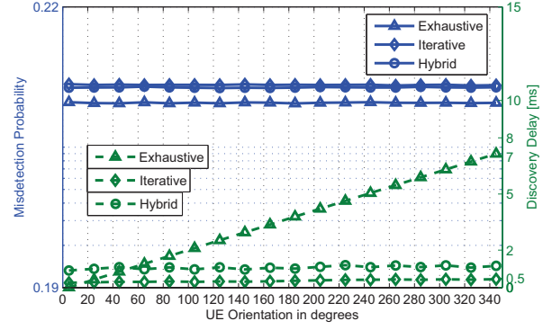
Fig. 4. UE orientation vs misdetection probability and discovery delay.
