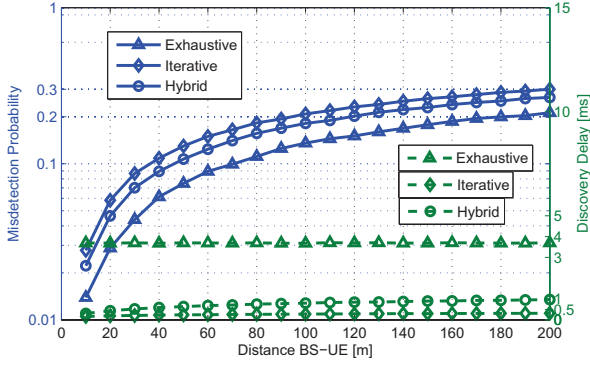
Fig. 3. Distance vs misdetection probability and discovery delay.
