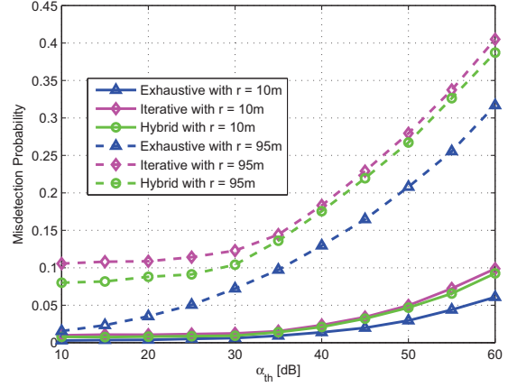
Fig. 1. Misdetection probability for the three algorithms at r = 10m and r = 95m .
