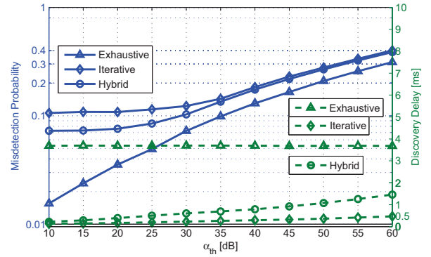
Fig. 2. SNR threshold vs misdetection probability and discovery delay.
