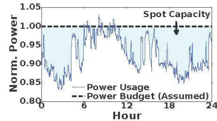
Figure 1: Power trace of a production server cluster in a top-brand IT company.
