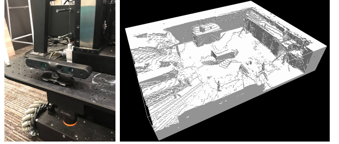
Fig. 5: Left: the PrimeSense depth camera mounted on the robot base. Right: one 8m×6m×1.5m occupancy grid map built by the mapper module.
