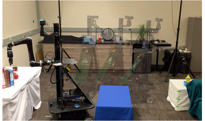
Fig. 1: The Vector mobile manipulator, with an omni-drive base and a 6-DOF Kinova JACO2 arm, is solving the STEAP problem. The task involves picking up an object from the white table on the right and dropping it off on the white table on the left, while avoiding the blue table. The semi-transparent robots show the trajectory taken, while the solid robot is the goal configuration.
