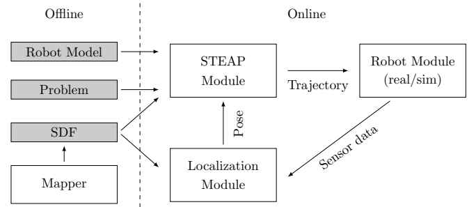
Fig. 4: Block diagram of our framework showing all the components and how they interact. White boxes are modules and gray boxes are data. Sensor measurements flow from Robot Module to Localization Module.
