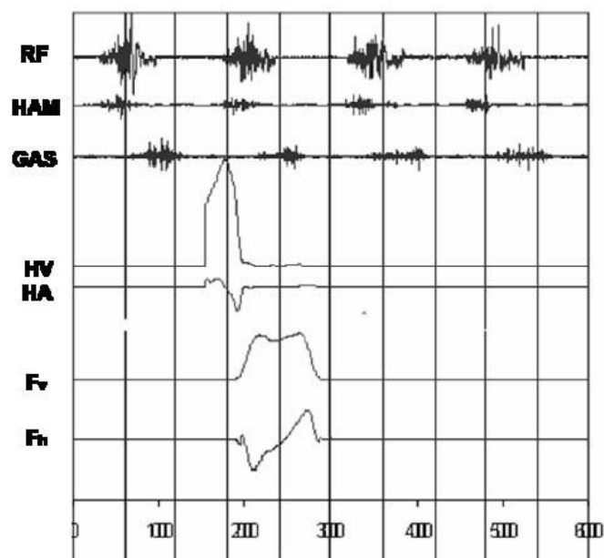
Figure 3. Composite view of raw EMG of rectus femoris (RF), hamstring (HAM), and gastronemius (GAS) muscles, heel velocity (HV), heel acceleration (HA), vertical force (Fz), and horizontal force (Fx).
