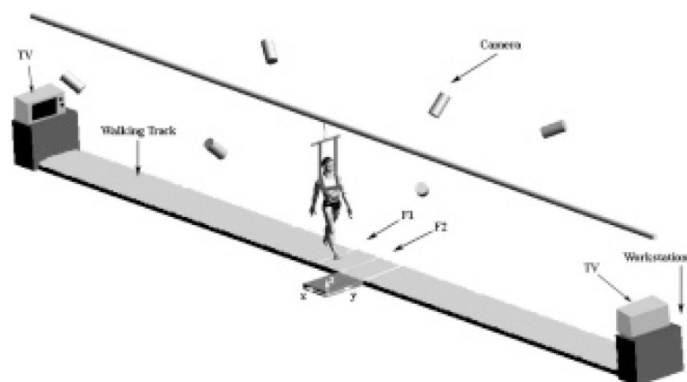
Fig. 1. Field layout of the experimental set-up including; Fall Arresting System, Infra-red cameras (6), Two force plate (F1 and F2), and workstations. X, Y, and Z=global references for force and position. The surface of F2 was used to created slipperiness.
