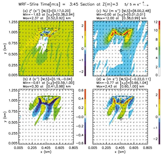
Fig. 10. Horizontal cross sections for 3 m a.g.l. of (a) horizontal x vorticity \zeta^x ( \text{s}^{-1} ), (b) horizontal divergence \delta ( \text{s}^{-1} ), (c) speed of horizontal wind |\mathbf{V}_H| ( \text{m s}^{-1} ), and (d) vertical velocity w ( \text{m s}^{-1} ) at 3:45 [min:s] into the WRF-SFIRE simulation. Magnitudes of each contour are indicated by colors in bar plots on the right. For each field, minimum and maximum values, plus their (x, y) positions on cross section are given. Vectors denote wind components in x – y plane where magnitude is scaled as indicated in the top right corner of plot. Black dotted contour lines delineate the surface fire perimeter. Note that the (aspect) ratio between the height of each plot to its width is not equal to one. Plots show features lengthened in the y direction compared to the x direction. The (x, y) locations of the MT and ST are indicated by black diamonds.
