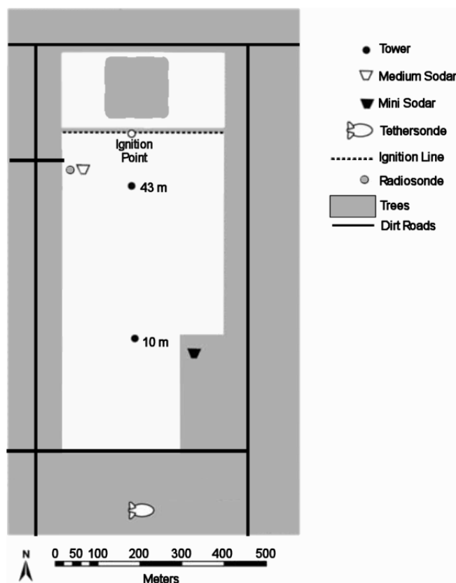
Fig. 1. Instrument locations and the layout of the FireFlux experiment. White area indicates grass.
