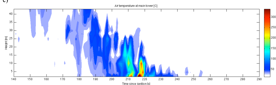
Figure 7. Air temperatures at the MT as a function of time: a) WRF-simulated, b) thermocouple 5 s averaged, c) thermocouple raw (1 s).
