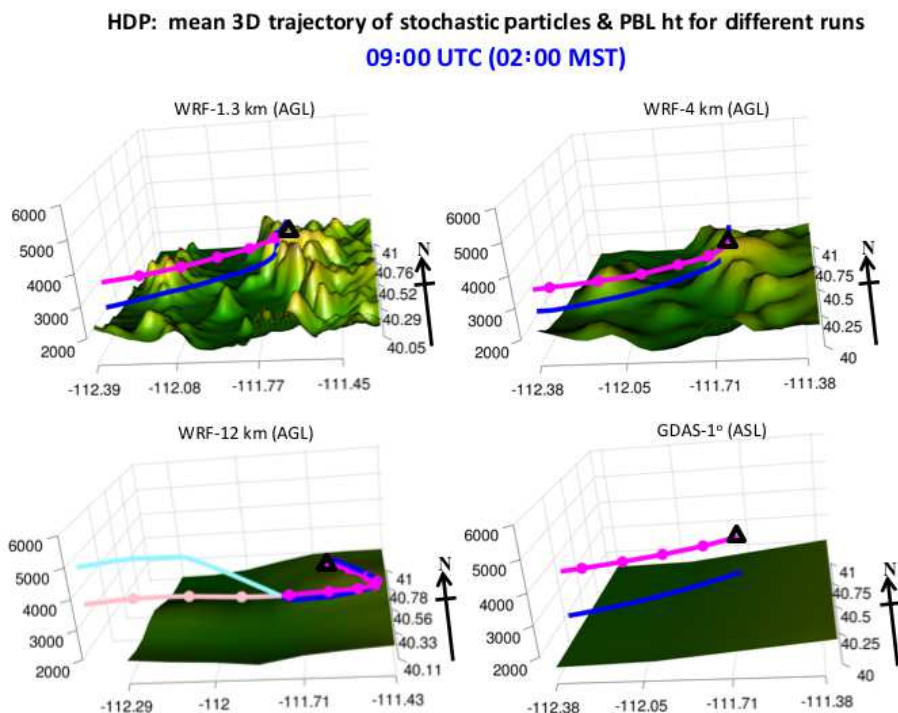
Figure 7. Three dimensional plots of the terrain over a domain of \sim 1^\circ \times 1^\circ surrounding HDP, as resolved by the WRF and GDAS models at various grid spacings. The HDP site is denoted as a triangle. Also shown is the average back trajectory, derived by averaging locations of the numerous stochastic trajectories simulated by STILT, driven by the various WRF meteorological fields and the global GDAS field. Back trajectories were started from HDP at 02:00 MST (09:00 UTC). Points indicate trajectory locations every hour, as the trajectory moves back from the site indicated as points. Magenta portions of the trajectory refer to the nighttime (19:00–07:00 MST), while pink portions indicate the daytime (07:00–19:00 MST). In addition, the PBL heights averaged along the back trajectory are shown as the blue line.
