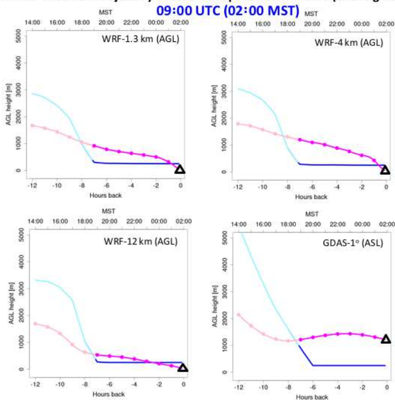
Figure 12. Similar to Fig. 10, but for the Niwot Ridge (NWR) site.
