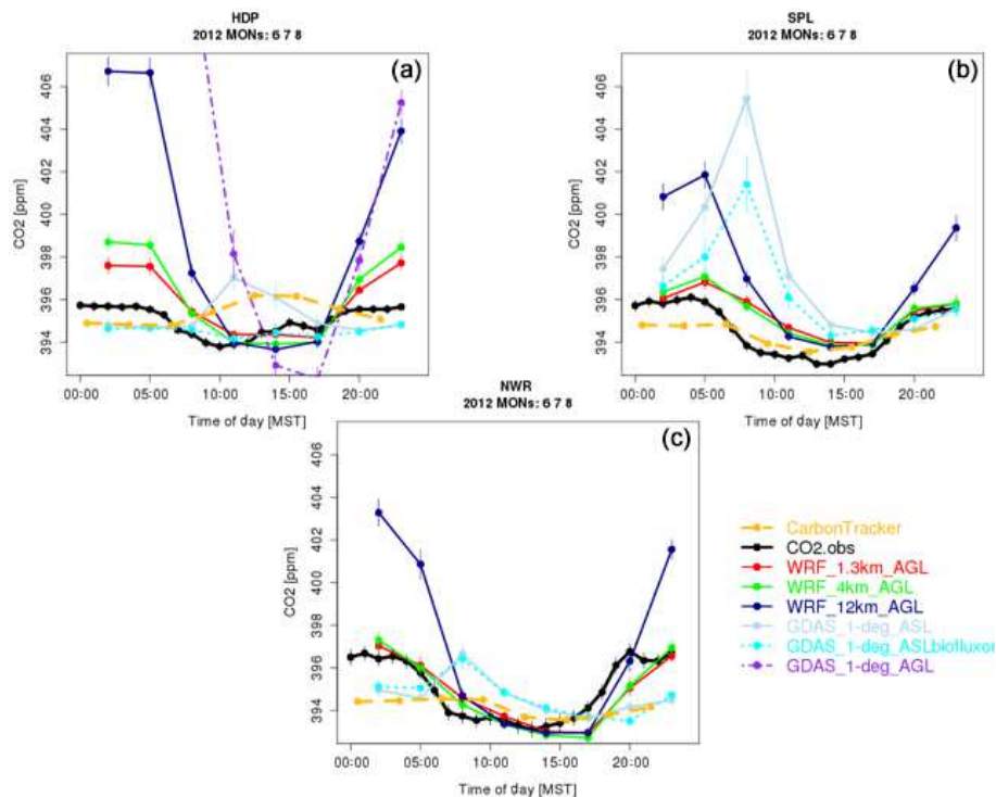
Figure 3. The average diurnal CO 2 pattern during June–August 2012 as observed at the three mountaintop sites in the RACCOON network: Hidden Peak (HDP), Storm Peak Laboratory (SPL), and Niwot Ridge (NWR). Compared against the observations are simulated diurnal CO 2 patterns from different models: CarbonTracker, STILT driven with WRF at different grid spacings, and STILT driven with GDAS. Multiple GDAS-driven STILT model configurations are shown, including runs without fixes to the biospheric fluxes (“biofluxorig”; see the Supplement) as well as releasing air parcels at the elevations of the sites above mean seal level (ASL) or, for HDP only, at the inlet height (Table 1) above the model’s ground level (AGL). All of the WRF-driven STILT runs place the release point of air parcels following the AGL configuration. Error bars denote standard errors of the diurnal averages.
