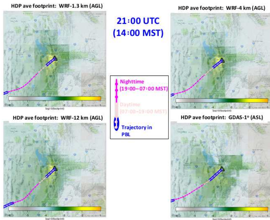
Figure 6. Similar to Fig. 5, but for the afternoon: 14:00 MST (21:00 UTC) at HDP.
