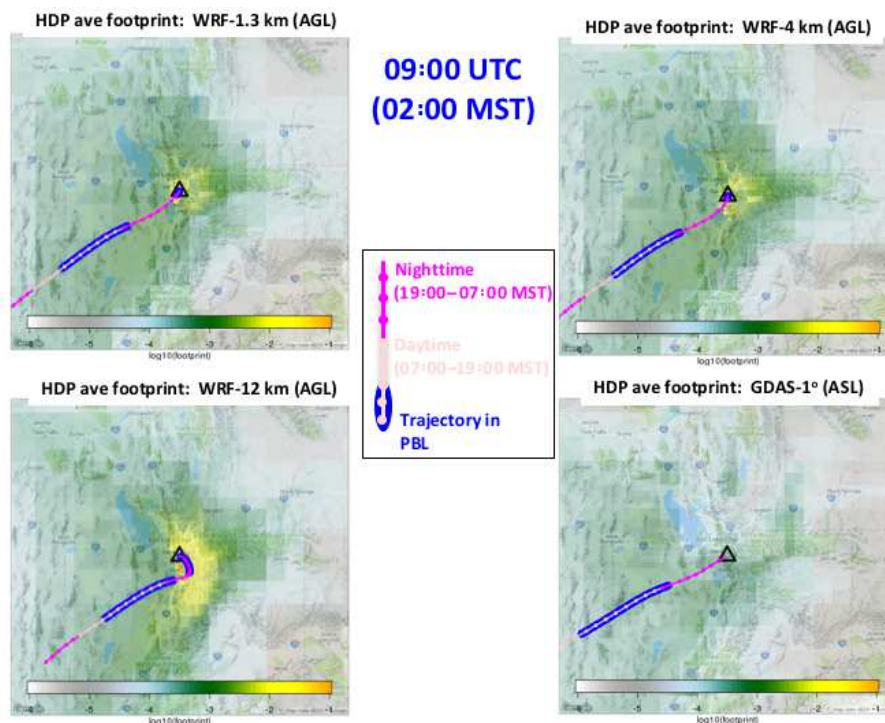
Figure 5. The average footprint (shown in \log_{10} ) for the Hidden Peak (HDP) site in Utah, at night: 02:00 MST (09:00 UTC), gridded at 0.1^\circ \times 0.1^\circ . The site is denoted as a triangle. The average back trajectory (averaged over the stochastic STILT trajectories) is drawn as a line, with points indicating trajectory locations every hour, as the trajectory moves back from the site indicated as points. Magenta parts of the trajectory refer to the nighttime (19:00–07:00 MST), while pink portions indicate the daytime (07:00–19:00 MST). Parts of the trajectory are shaded with blue when it is found below the average height of the PBL along the trajectory.
