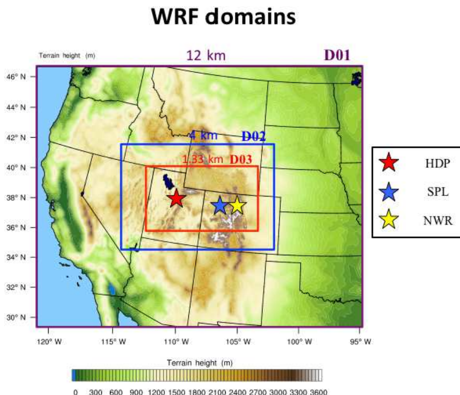
Figure 2. The WRF simulation domain, covering the western US with a series of nests with 12, 4, and 1.3 km grid spacing. These WRF meteorological fields are used to drive air parcel trajectories within the STILT model.
