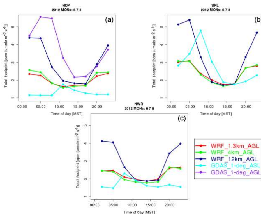
Figure 4. The average diurnal footprint strengths at HDP, SPL, and NWR over June–August 2012 from STILT, driven with different meteorological fields and release heights (ASL vs. AGL). The footprint strength was derived by summing over the spatial distribution of footprint values (Fig. 5).
