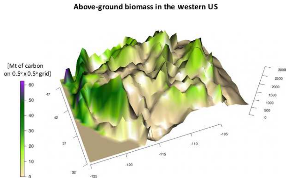
Figure 1. Above-ground biomass (megatons, Mt, of carbon) from the North American Carbon Program baseline dataset for year 2000 (Kelldorfer et al., 2013) overlaid on topographic surface in the western US, resolved at 0.5^\circ \times 0.5^\circ grid spacing.
