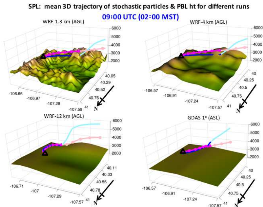
Figure 9. Similar to Fig. 7, but for the Storm Peak Laboratory (SPL) site.
