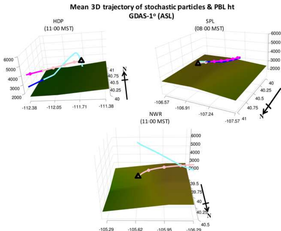
Figure 13. Similar to three-dimensional terrain and trajectory plots as shown in Figs. 7, 9, and 11, but for just the GDAS 1°. ASL simulations and for the morning hours of 08:00 and 11:00 MST.
