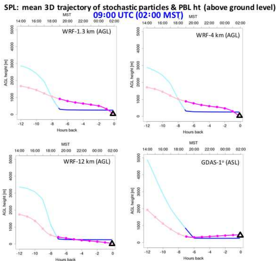
Figure 10. Similar to Fig. 8, but for the Storm Peak Laboratory (SPL) site.
