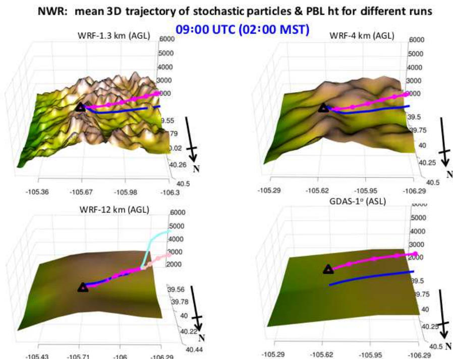
Figure 11. Similar to Fig. 9, but for the Niwot Ridge (NWR) site.
