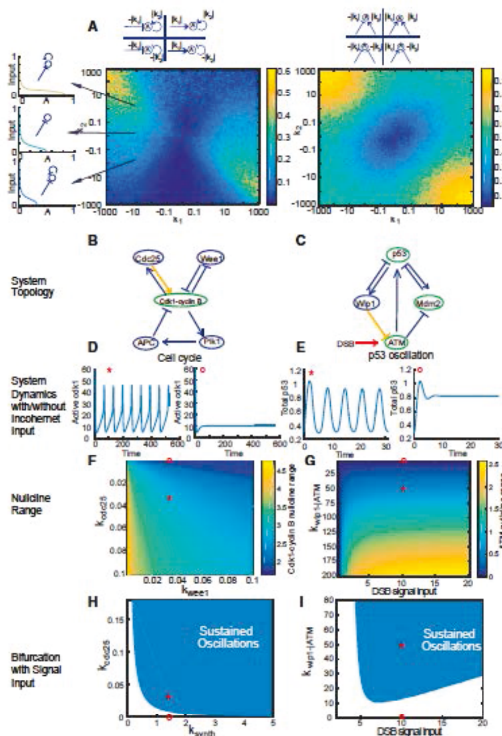
Figure 3. Incoherent Inputs Improve the Robustness of Biological Oscillators with Experimentally Estimated Parameters
