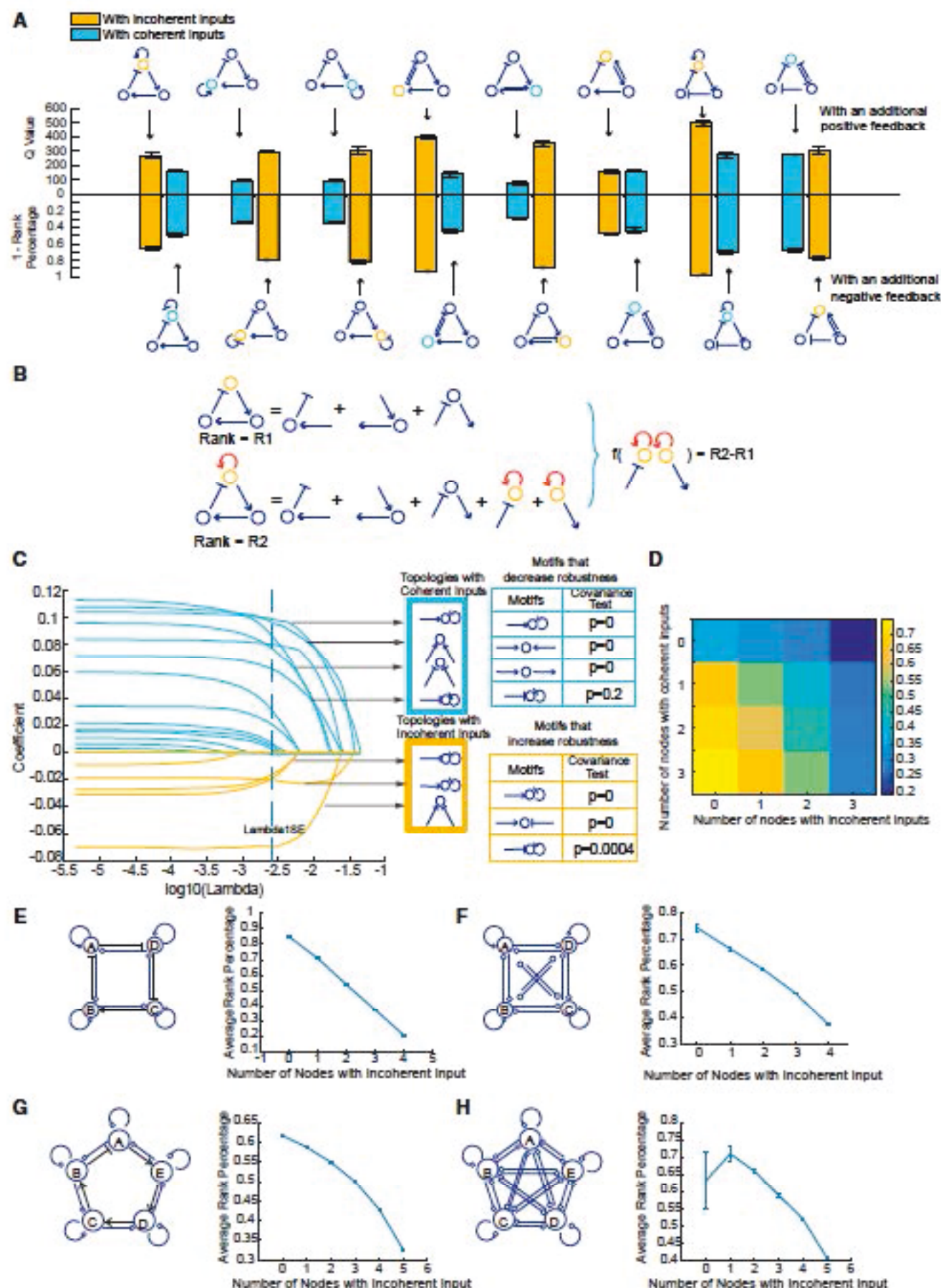
Figure 2. Incoherent Inputs Significantly Increase the Overall Robustness of an Oscillator
