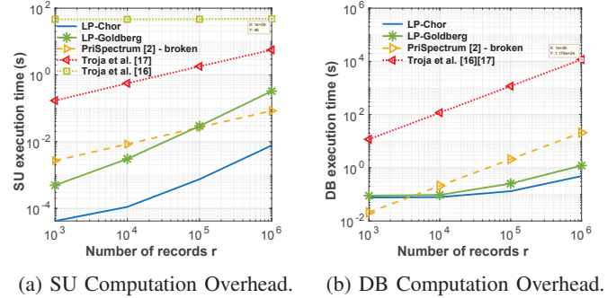
(a) SU Computation Overhead. (b) DB Computation Overhead.
