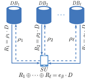
Fig. 1: Main steps of LP-Chor Algorithm
