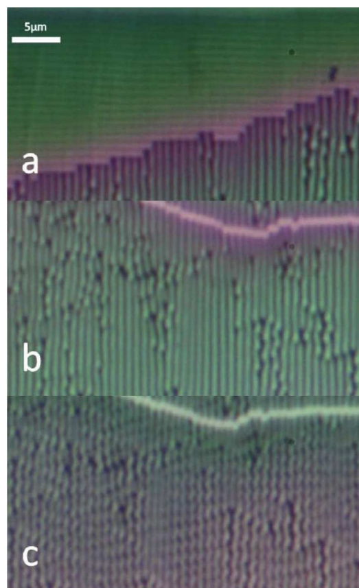
Fig. 6 Photomicrographs of soapy streaks that formed from 9004 on RN1175 at T_{AC} - T a) 0.1, b) 4.3, and c) 7.4 K. All images were taken at the same location. The 5 \mu\text{m} scale bar is oriented perpendicular to the easy axis and the polarizer is at 45^\circ with respect to the scale bar. Film thickness is \sim 250 nm.
