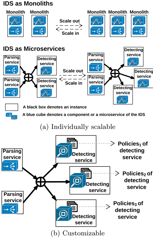
Figure 2: Benefits of IDS virtualization as microservices
