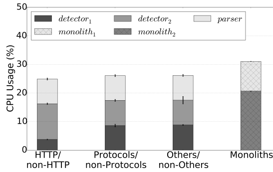
Figure 3: CPU usage of different microservice instances compared with that of monolithic instances. The HTTP/non-HTTP, Protocols/non-Protocols and Others/non-Others are the emulation results of three different methods to partition the detection policies. The Monoliths are the experimental results of the two monolithic Bro instances.
