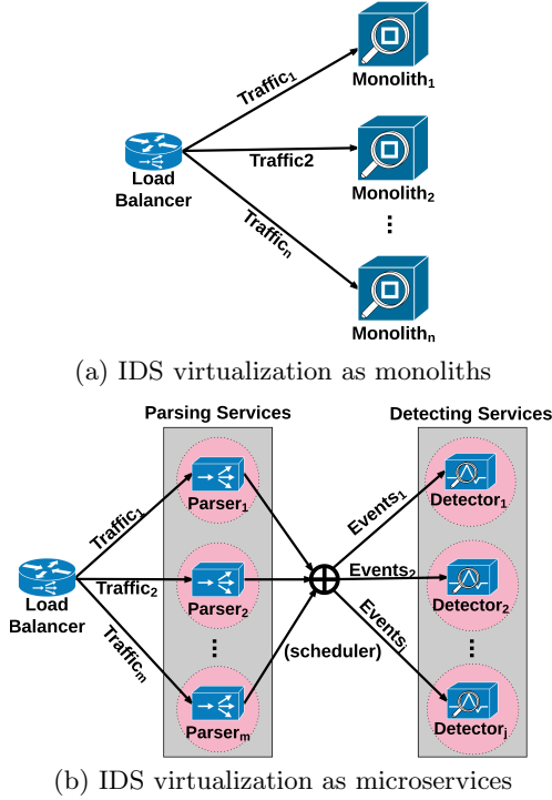
Figure 1: IDS virtualization as monoliths and microservices
