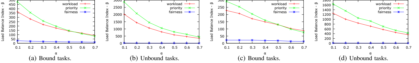
Figure 7: Load balance index in the case of bound (a) and unbound (b) tasks with log-uniform runtimes; and in case of bound (c) and unbound (d) tasks with uniform runtimes.
