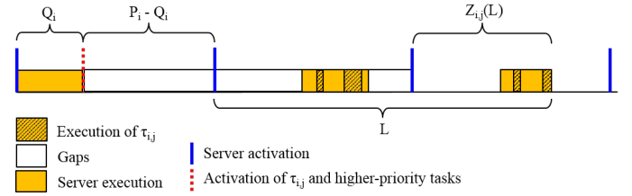
Figure 4: Critical instant scenario for an unbound task scheduled under a periodic server.
