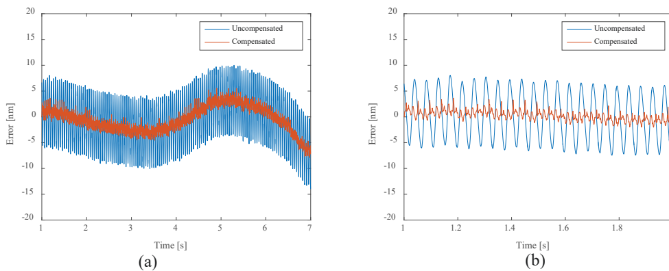
Fig. 9. (a) The result of periodic error compensation for the experimental constant velocity motion, and (b) zoomed view of the compensation result.
