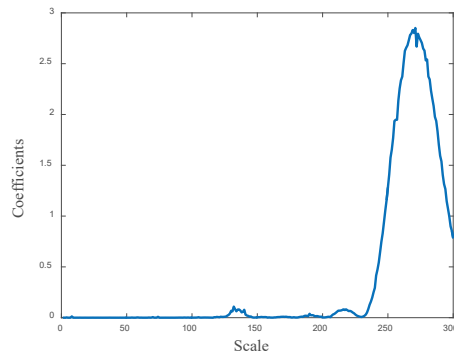
Fig. 7. An example of finding the ridge from wavelet transform coefficients at 7 s.
