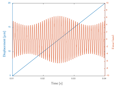
Fig. 4. Simulated displacement and periodic error.
