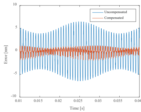
Fig. 5. Periodic error compensation result for the simulated motion.
