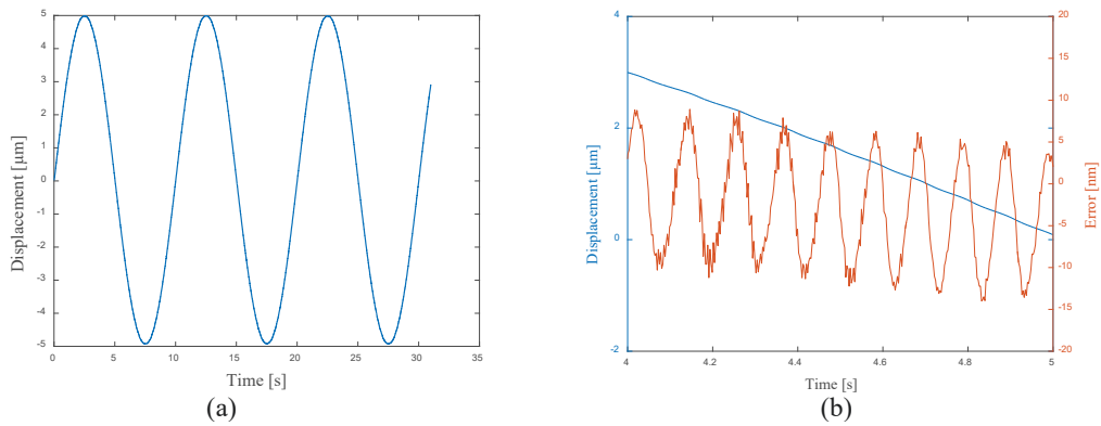
Fig. 10. (a) The experimental reciprocal displacement, and (b) zoomed view of the displacement and superimposed periodic error.
