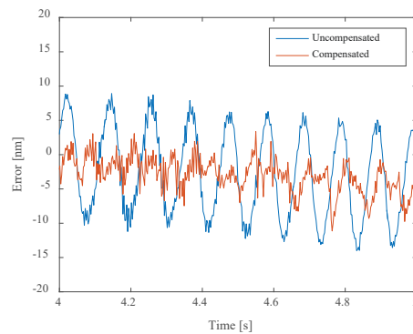
Fig. 11. Periodic error compensation result for the experimental non-constant velocity motion.
