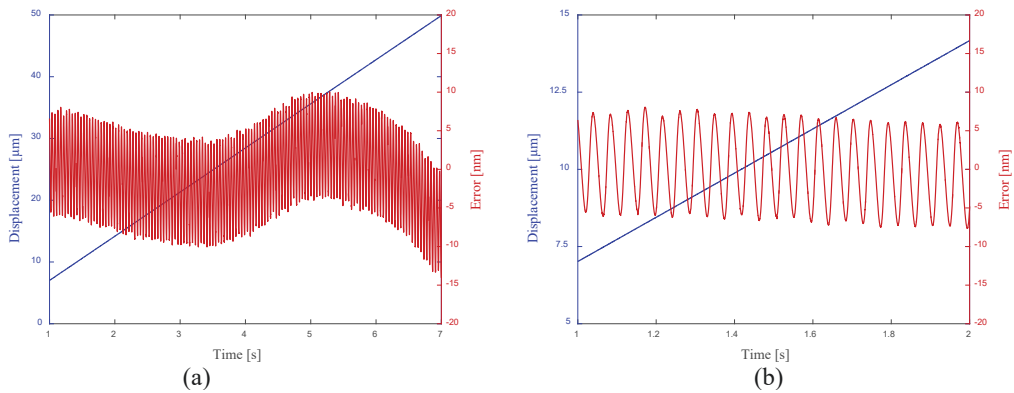
Fig. 6. (a) Experimental linear displacement and periodic error, and (b) zoomed view of the displacement and superimposed periodic error.
