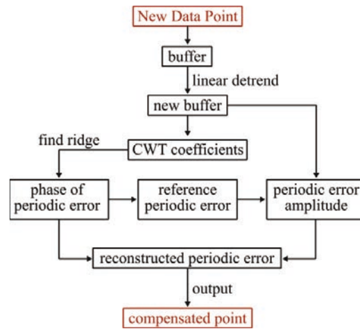
Fig. 2. Calculations to implement the periodic error compensation algorithm.
