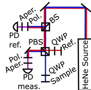
Fig. 16. The optical layout of the heterodyne interferometer used for testing. Apertures (aper.) are used to set the level of periodic error.
