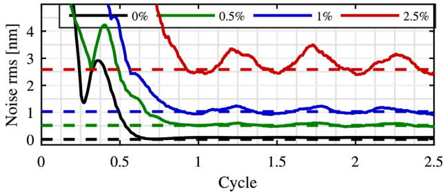
Fig. 15. The RMS of the residual noise in output when adding different levels of noise to input signals. The solid lines are the local RMS of 50 points of residual noise after correction. Using local RMS instead of global RMS eliminates the influence of transient state at the beginning. The dash lines are the levels of input noise. Because the Kalman filter in this design only deals with periodic error, the white noise in the inputs will pass through and be left in the output.
