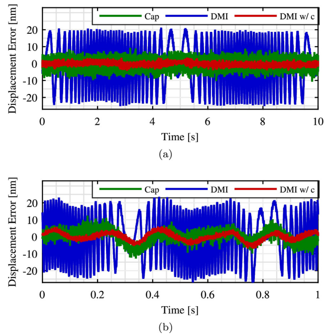
Fig. 18. Measurement error comparison among capacitive sensor, interferometer, and interferometer with error correction. (a) Illustrates the residual errors when measuring a sinusoidal motion: 5\mu\text{m} \cdot \sin(2\pi \cdot 0.1\text{Hz} \cdot t) . (b) Illustrates the residual errors when measuring a sinusoidal motion: 5\mu\text{m} \cdot \sin(2\pi \cdot 1\text{Hz} \cdot t) .
