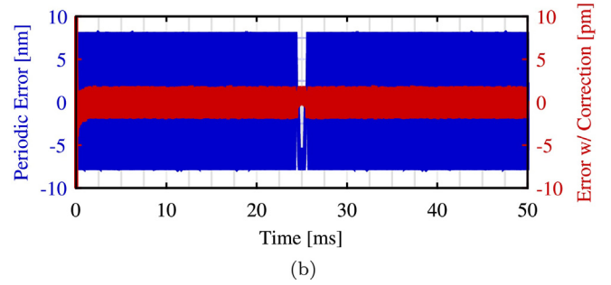
Fig. 13. Comparison of periodic error before and after correction, when the Doppler frequency is oscillating at 100 Hz. When the peak Doppler frequency is 1.99 kHz (0.63 mm/s) (a), the periodic error attenuates from \pm 8.0 nm to \pm 2.1 pm, RMS attenuates from 4.5 nm to 0.6 pm. When the peak Doppler frequency is 49.6 kHz (15.7 mm/s) (b), the periodic error attenuates from \pm 8.0 nm to \pm 2.3 pm, RMS attenuates from 4.7 nm to 0.7 pm.
