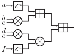
Fig. 6. The architecture of operation set 1. And it takes 7 clock cycles from input to result.
