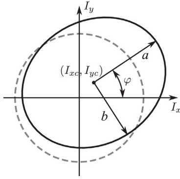
Fig. 3. The Lissajous curve of raw (I_x, I_y) (ellipse) and corrected (I_x, I_y) (circle). For those coefficients in ((8, 9)), I_{xc} and I_{yc} are the center of ellipse, a and b are major and minor semi-axes, and \varphi is the angle between the X-axis and the major axis. The goal of ellipse fitting is to eliminate the influence of DC offset, unequal gain and quadrature phase shift.
