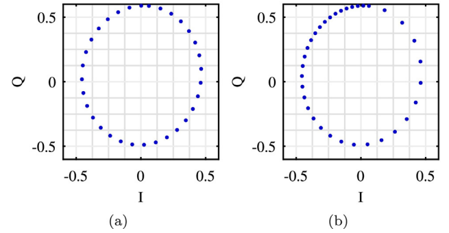
Fig. 10. Doppler frequency influences the distribution of samples on Lissajous curve. (a) and (b) show the Lissajous curves of in-phase (I) and quadrature (Q) signals of the measurements with periodic error. Constant Doppler frequency leads even distribution (a), and non-constant Doppler frequency leads uneven distribution (b).
