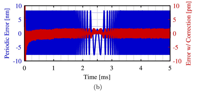
Fig. 14. Comparison of periodic error before and after correction, when the Doppler frequency is oscillating at 10 Hz. When the peak Doppler frequency is 1.99 kHz (0.63 mm/s) (a), the periodic error attenuates from \pm 8.0 nm to \pm 2.2 pm, RMS attenuates from 5.2 nm to 0.6 pm. When the peak Doppler frequency is 49.6 kHz (15.7 mm/s) (b), the periodic error attenuates from \pm 8.0 nm to \pm 2.1 pm, RMS attenuates from 4.6 nm to 0.7 pm.
