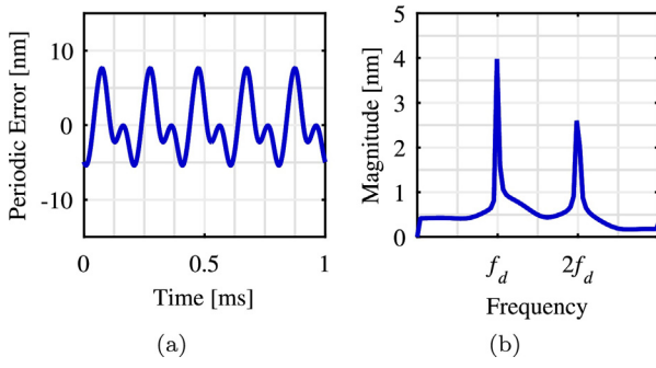
Fig. 2. The periodic error of displacement in time domain (a) and frequency domain (b) when simulating a constant velocity motion. In time domain, the overall periodic error is usually on the order of nanometer. In frequency domain, the two orders of periodic error locate at Doppler frequency and two times of Doppler frequency, respectively. If the motion is non-constant velocity, the two peaks will keep shifting on the spectrum. It is impractical to use Fourier transform to characterize the periodic error in a long period.
