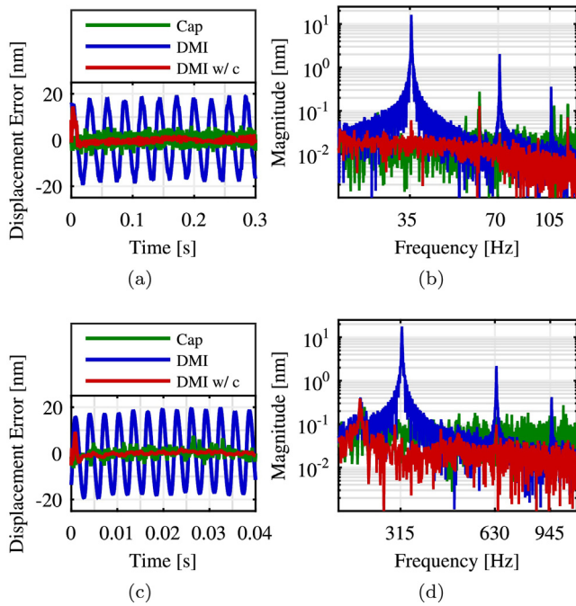
Fig. 17. Measurement error comparison among capacitive sensor, interferometer, and interferometer with error correction. (a) and (b) are the residual error and its spectrum for 11\mu\text{m/s} motion (Doppler frequency 35 Hz) measurement. After correction, the first- and second-order error attenuate 48.5 dB and 36.5 dB, respectively. (c) and (d) are the residual error and its spectrum for 99.7\mu\text{m/s} motion (Doppler frequency 315 Hz) measurement. After correction, the first- and second-order error attenuate 51.1 dB and 26.9 dB, respectively.
