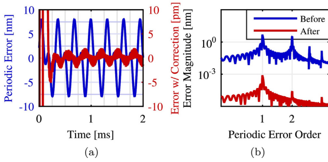
Fig. 11. Comparison of periodic error before and after correction. The Doppler frequency is 3.16 kHz. In the time domain (a), the periodic error attenuates from \pm 8.0 nm to \pm 2.1 pm, RMS attenuates from 4.7 nm to 0.7 pm. In the frequency domain (b), the first- and second-order error attenuate 75.9 dB and 102.0 dB, respectively.
