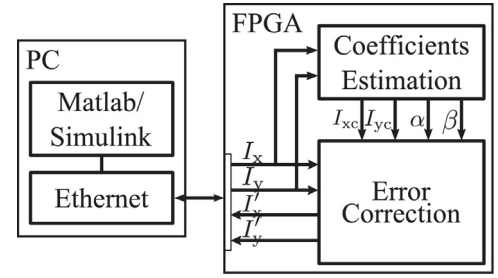
Fig. 9. The setup of HIL simulation. On PC side, Stimulus is generated by Matlab/Simulink, and transmitted to FPGA by Ethernet. On FPGA side, the stimulus is processed by periodic error correction module, and the result is transmitted back to PC for further processing and analysis.
