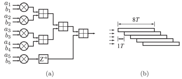
Fig. 7. (a) The architecture of operation set 2. Its function is to calculate the summary of five results of multiplication, which is a common operation set in matrix multiplication. The internal signals are exactly synchronous. (b) The timing for operating this set. It is pipelined, so at each clock it could have a new data in. And it takes 8 clock cycles from input to result.
