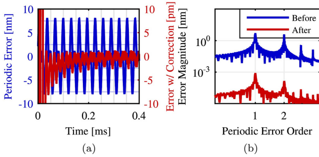
Fig. 12. Comparison of periodic error before and after correction. The Doppler frequency is 31.6 kHz. In the time domain (a), the periodic error attenuates from \pm 8.0 nm to \pm 2.1 pm, RMS attenuates from 4.7 nm to 0.7 pm. In the frequency domain (b), the first- and second-order error attenuate 76.2 dB and 88.4 dB, respectively.
