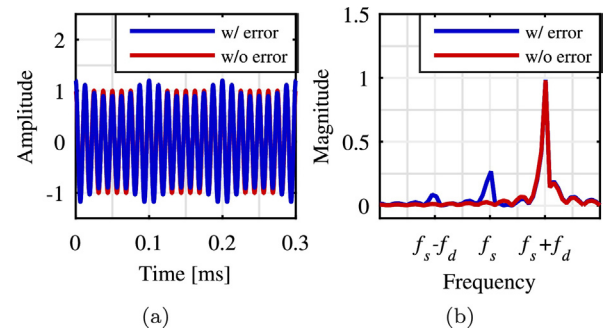
Fig. 1. The measurement signal I_m in time domain (a) and frequency domain (b) when simulating a constant velocity motion. In the time domain, the amplitude of the measurement signal is varied, due to the appearance of periodic error. In the frequency domain, two extra peaks appear, represent first- and second-order periodic error respectively, whose frequencies are related to the Doppler frequency f_d , and split frequency f_s [27].
