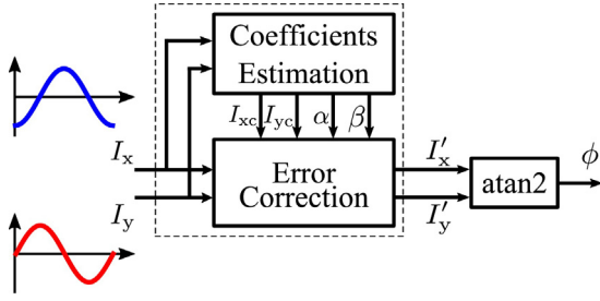
Fig. 5. The structure of periodic error correction module. It extracts the correction coefficients from the input in-phase and quadrature signals and applies the coefficients back to the signals for correction.
