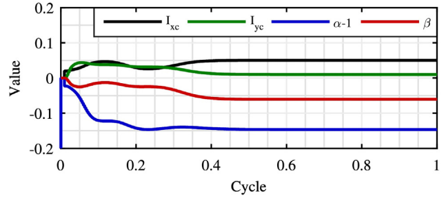
Fig. 4. The correction coefficients converge within half of the cycle.
