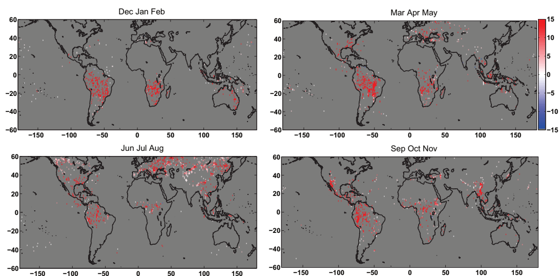
Figure 3. Difference between lightning densities observed on polluted and clean days, for the four seasons of 2012. The gray areas contain insufficient data for analysis or failed the t -test (at the 95% confidence level).
