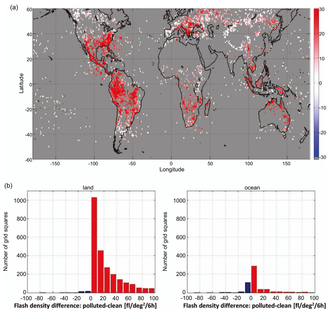
Figure 2. (a) Global map of differences between flash densities observed on polluted and clean days for 2012. The gray areas contain insufficient data for analysis or failed the t -test (at the 95% confidence level). (b) Histograms of the differences between flash densities on polluted and clean days [fl/deg 2 /6 hr] for land (left) and ocean (right).
