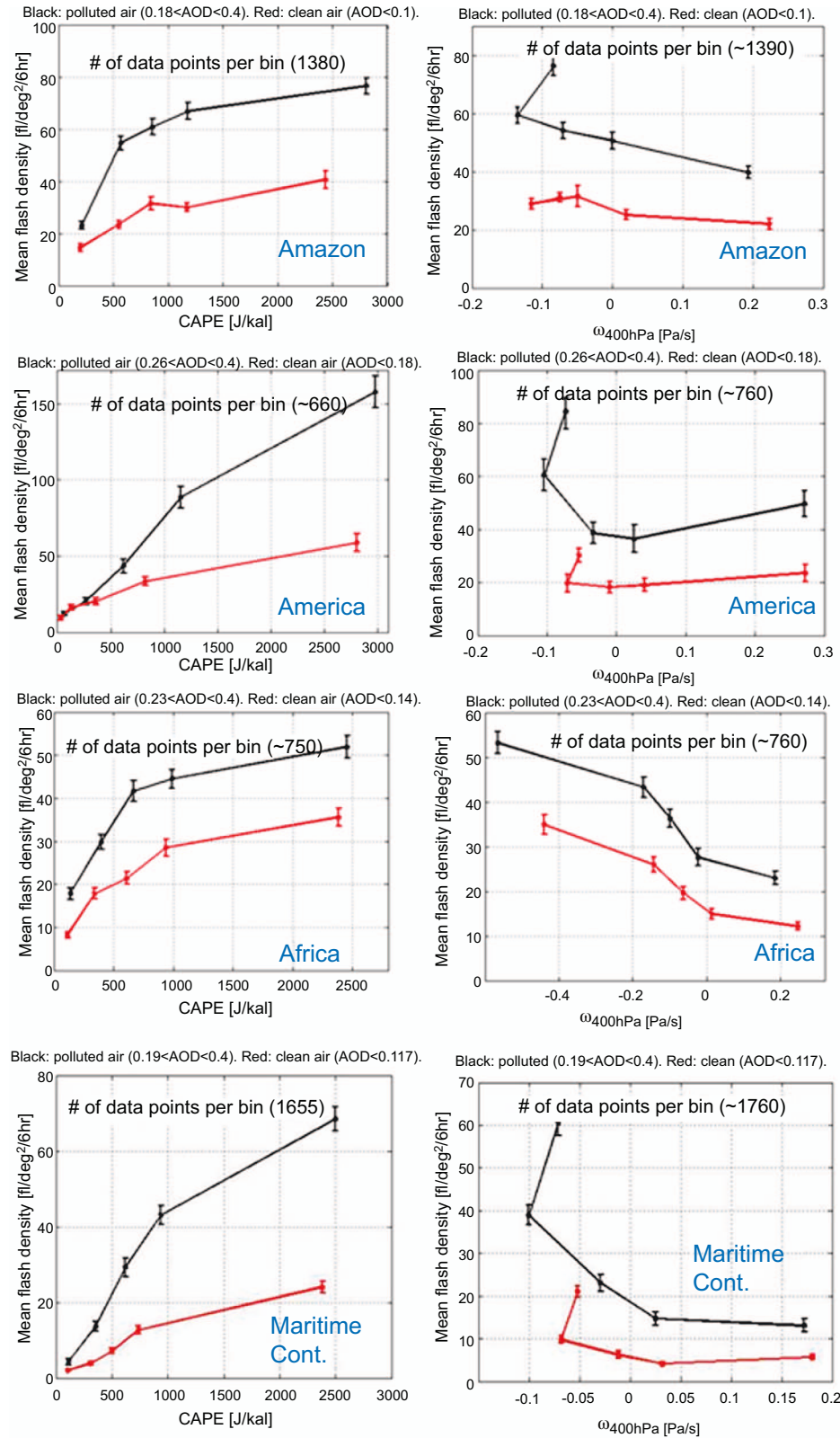
Figure 4. Mean flash density as a function of CAPE (left column), \omega_{400\text{ hPa}} (right column), for clean (red curves) and polluted (black curves) conditions for the Amazon (March–May 2012, 14 LT, upper row), North America (June–August 2012, 13 LT, second from top row), southern Africa (January–February, and December 2012, 14 and 17 LT, third from top row) and the Maritime Continent (March–May 2012, 14 LT, bottom row). The specified values of AOD ranges and the numbers of analyzed data points (per bin) appear in each panel. Error bars represent the standard deviation within each interval. Black curves exceed the red ones everywhere.
