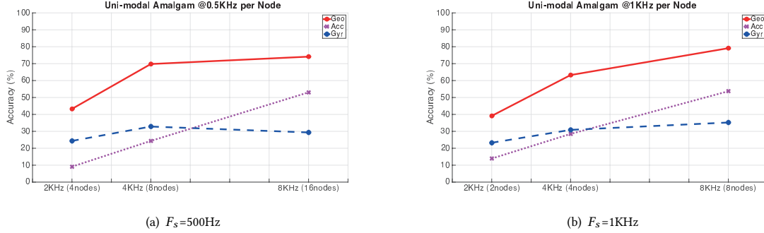
Figure 9: Amalgam signals constructed with F_s=500\text{ Hz} and 1\text{KHz} for Figure 9(a) and 9(b), respectively. Recognition accuracy of each Amalgam signal increases as F_{s\_Amal} increases from 2, 4, and 8 KHz by varying number of nodes from 4, 8, and 16 for Figure 9(a), and 2, 4, and 8 for Figure 9(b), respectively
