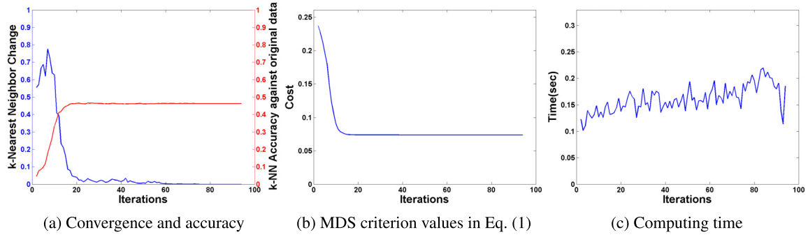
Figure 2: Iteration-wise behavior of MDS for 500 handwritten digit data represented in 16 dimensions.
