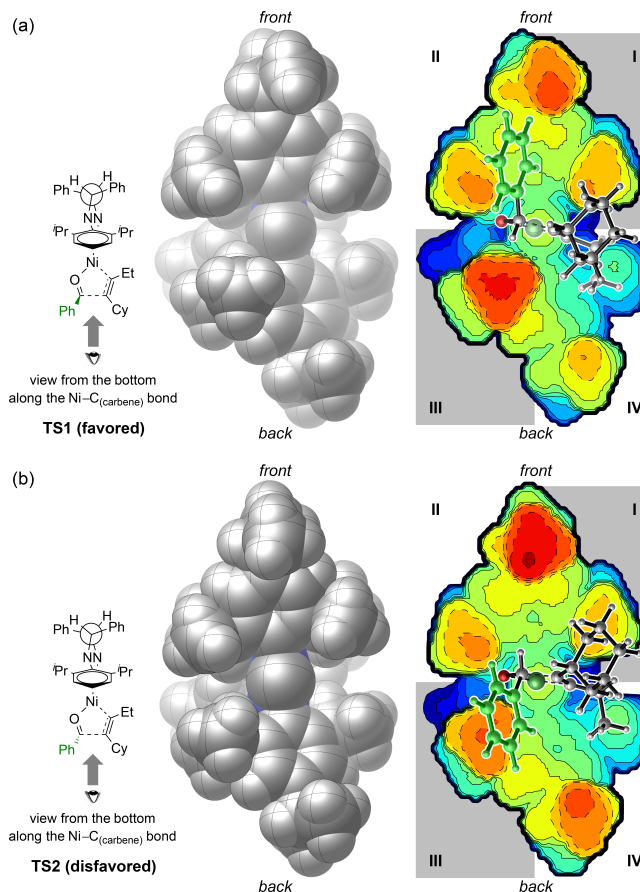
Figure 2. van der Waals surface and steric contour plot of ligand 4b in the oxidative cyclization transition states TS1 and TS2. The geometries of the benzaldehyde and the alkyne are overlaid onto the contour plots. Red and yellow in the contour plots indicate regions that are occupied by the NHC ligand.
