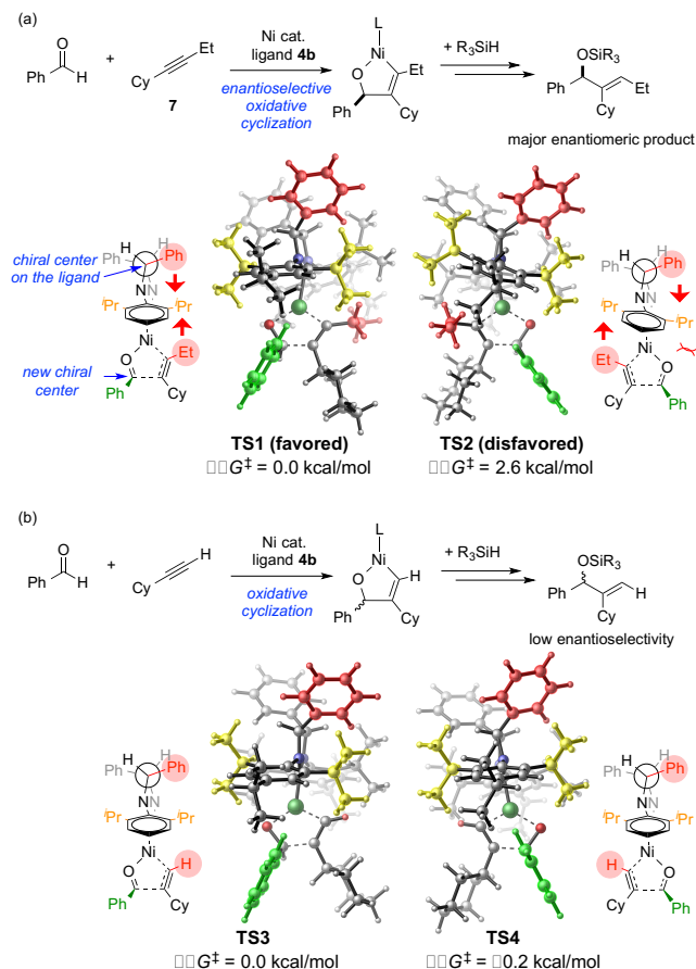
Figure 1. Remote chiral induction by the C2 symmetric ligand 4b in the oxidative cyclization transition states. Energies are computed at the M06/SDD-6-311+G(d,p)/SMD (toluene) level of theory with geometries optimized at the B3LYP/LANL2DZ-6-31G(d) level.
