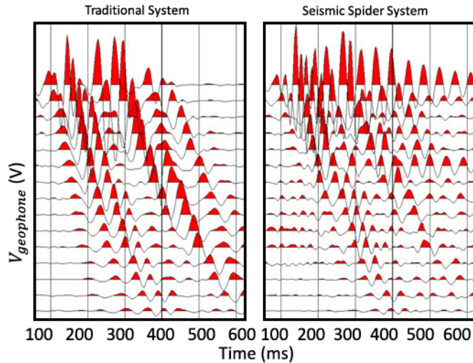
Fig. 9. Shot gather comparison of traditional geophones versus SeismicSpider.
