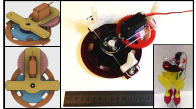
Fig. 11. Deployment system for dropping SeismicDarts from the UAV. Pictured design holds four darts, but can be scaled according to the UAV's carrying capacity.
