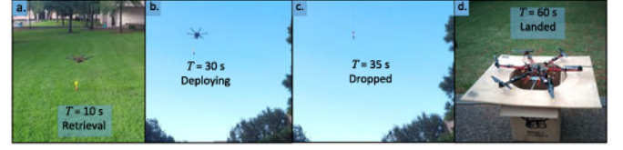
Fig. 7. SmartDart retrieval and redeployment. See video attachment.
