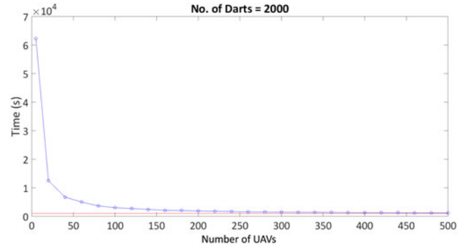
Fig. 16. Survey time for a 1 \text{ km} \times 10 \text{ km} region for different numbers of UAVs.
