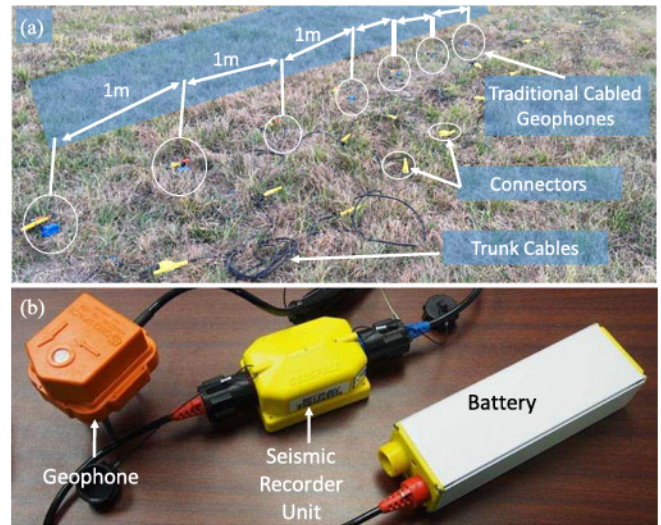
Fig. 2. Comparing state-of-the-art seismic survey sensors. (a) A traditional cabled system connects geophones in series to a seismic recorder and battery. (b) Autonomous nodal systems give each geophone a seismic recorder and battery.
