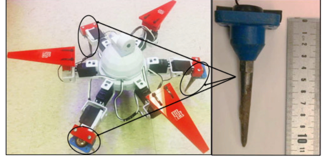
Fig. 8. The SeismicSpider is a six-legged mobile robot where geophones replace three legs. It is drone deployable, can sense and record seismic data, and can move to desired locations, including terrain the SeismicDart cannot access.
