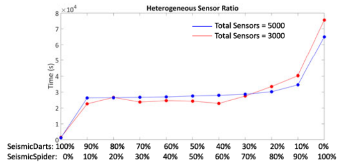
Fig. 17. Survey time for different sensor ratios. The total number of sensors {5000, 3000} were kept constant. Ten darts were provided for each UAV.
