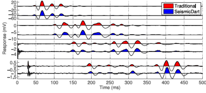
Fig. 6. Raw voltage data from shot gather comparison of four traditional geophones and four autonomously dropped SeismicDart sensors.
