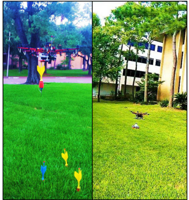
Fig. 1. The heterogeneous sensor system presented in this paper: wireless SeismicDarts and a SeismicSpider, both designed for UAV deployment.
