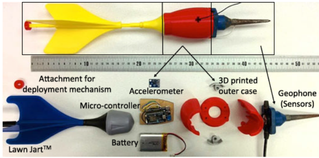
Fig. 3. Components of the SeismicDart sensor: a lawn Dart fin, particle.io Photon micro-controller, 3D printed protective casing, and a geophone.
