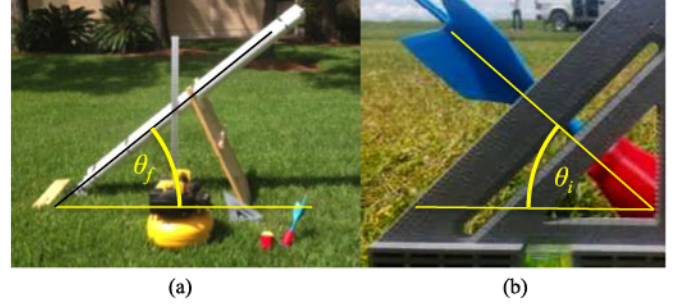
Fig. 14. A pneumatic launcher for SeismicDarts. Ballistic dart deployment has limited usefulness because the incident angle is equal to the firing angle.
