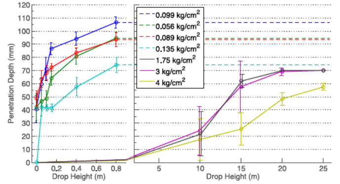
Fig. 4. Drop height versus penetration depth in seven soil types. Drops were performed autonomously and each data point represents 12 trials. Increasing the drop height increased the penetration depth for all seven soil types.
