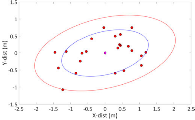
Fig. 13. Targeting accuracy. Circles show landing locations of 24 darts, each commanded to drop at the same GPS location. The mean position is marked by a diamond, ellipses show \sigma and 2\sigma covariance.
