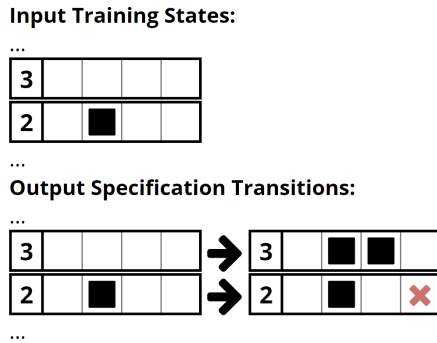
Figure 4: Example of the inputs and outputs for specification mining in our toy problem. Given a set of states, we use the rules of Nonograms to calculate deducible transitions for those states. Each transition serves as the specification for a potential rule.
