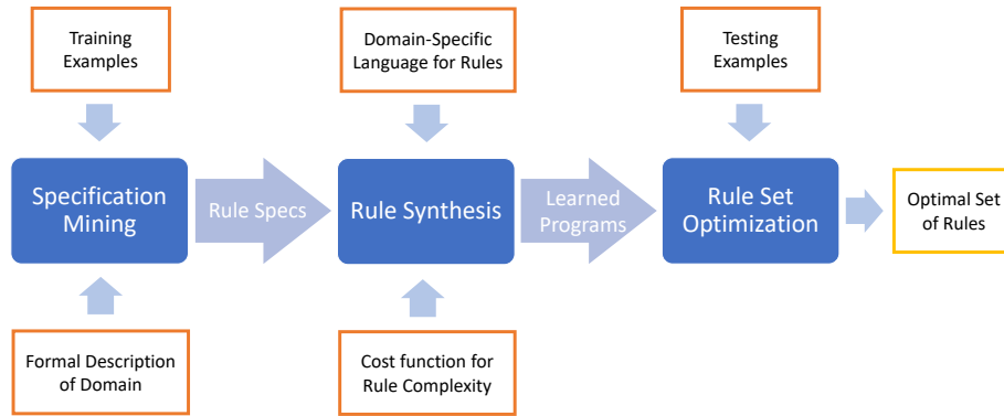
Figure 3: An overview our system’s three phases, along with their inputs and outputs.
