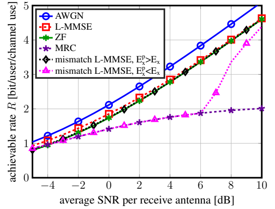
Fig. 2. Achievable rates for different equalizers with \beta = 0.3 . Overestimating ( E_x^p > E_x ) and underestimating E_x^p < E_x the signal power in the L-MMSE equalizer entails significant losses in terms of the achievable rates.
