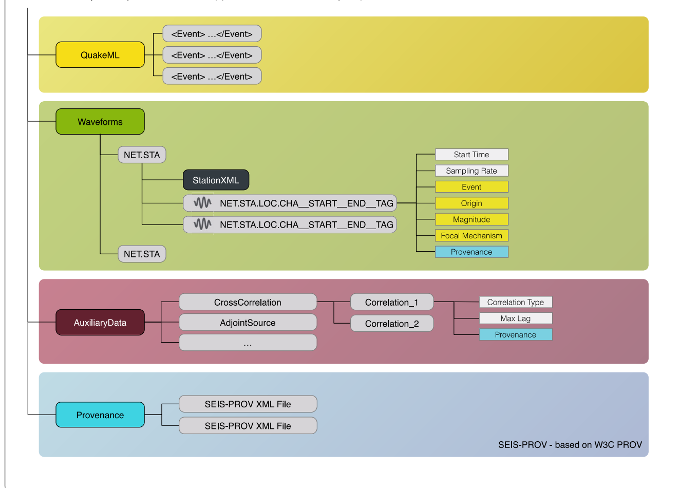
Figure 1. The general structure of an ASDF file in its HDF5 container—it has four distinct parts: (1, yellow) Information about an arbitrary number of earthquakes (or other seismic events) is stored in a single QuakeML document, the most complete earthquake description format currently available. (2, green) Seismic waveforms are stored per station together with the necessary meta information in the form of an FDSN StationXML document. (3, red) Anything that cannot be regarded as a seismic waveform is hierarchically stored in the auxiliary data section. (4, blue) Provenance information is stored as a number of SEIS-PROV documents, an extension to W3C PROV. Background colours in the attributes (rectangular boxes) denote relations to other sections in an ASDF file. Examples of this are relations of a waveform to a certain event or a provenance record for a piece of auxiliary data.
