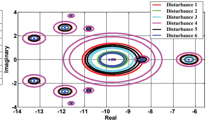
Fig. 4 Geršgorin disks due to disturbances shown in Table I
