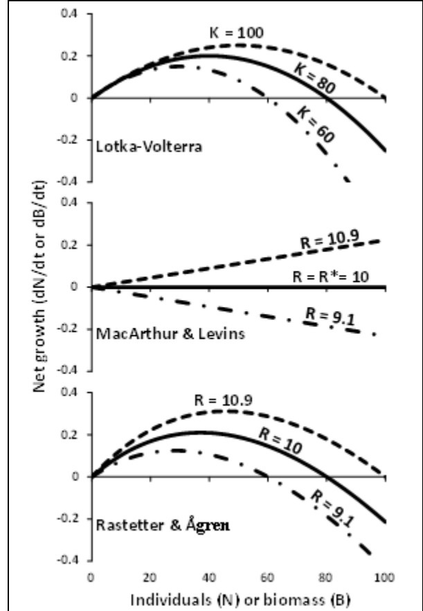
Figure 1: Comparison of net growth versus species abundance for Eqs. 1, 2, and 5. Upper panel- Lotka (1925) and Volterra (1926) model (Eq. 1) with r_i = 0.01 , \alpha_{ii} = 1 , and \alpha_{ji} = 0 for j \neq i . Middle panel - MacArthur and Levins (1964) model (Eq. 2) with g_i = 0.1 , k_{ij} = 10 , and m_i = 0.05 and R = the most limiting resource is held constant at the specified value. Lower panel - Rastetter and Ågren (2002) model (Eq. 5) with g_i = 0.125 , k_{ij} = 10 , and m_i = 0.05 , \alpha_i = 0.001 , \gamma_i = 0.00431 , and R = the most limiting resource is held constant at the specified value.
