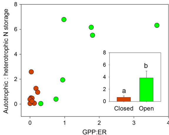
Fig. 6. Relationship between the ratio of autotrophic:heterotrophic N storage and GPP:ER. The inset shows the mean ( \pm SE) of the ratio of autotrophic:heterotrophic N storage for open- and closed-canopy streams. Different letters indicate differences in the mean ( \pm SE) between categories of stream canopy cover ( t test, P = 0.003 , t = -3.406 ) with brown (dark) and green (light) symbols representing open- and closed-canopy streams, respectively. See Table 1 for stream IDs.
