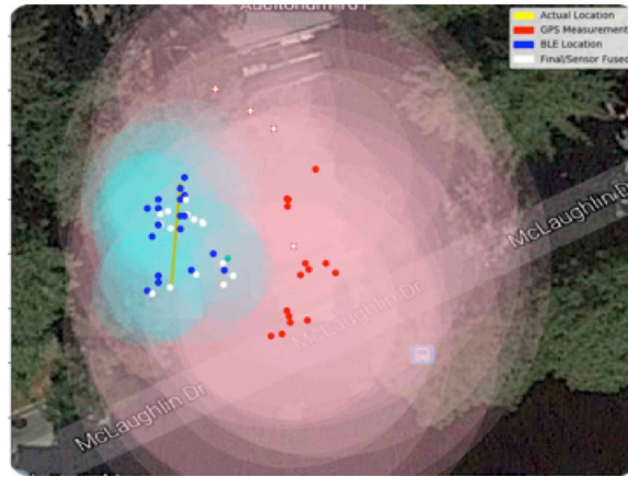
FIGURE 6 Location estimates and confidence circles computed at different times while the traveler was walking along the straight path represented by the yellow segment. Blue: beacons; red: GPS; white: statistical fusion of localization from beacons and GPS.
