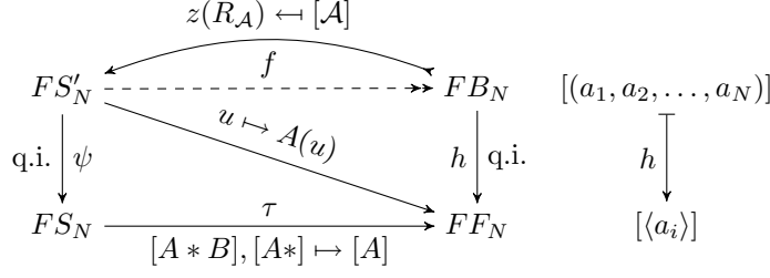
FIGURE 1. A diagram showing the maps between the various curve complex analogs considered in this paper. Here F_N = A* represents an HNN-extension splitting of F_N with the trivial associated subgroups and with the base group A . The map \psi is the quasi-isometry between FS'_N and FS_N given by the inclusion map.
