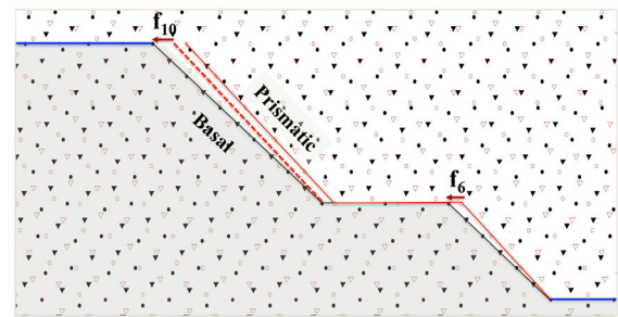
Figure 11. Schematic illustration of PB facets on a normal-TB viewed in the -\lambda = [\bar{1}\bar{1}20] direction. Facets with variable height form with disclination character represented by Frank vectors. \xi points toward the reader.
