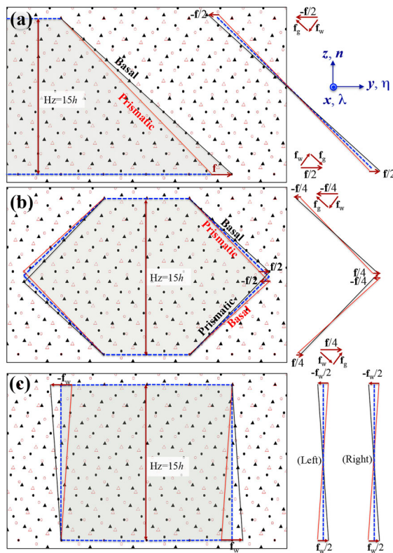
Figure 5. CDCs for a (\bar{1}0\bar{1}2) twin viewed in the -\lambda = [\bar{1}2\bar{1}0] direction, showing three type of forward boundaries: (a) an inclined boundary bonding the prismatic and basal planes that have a disclination angle of \varphi = 3.71 degrees, (b) two inclined boundaries with characteristic angles of \varphi = 3.71 and -3.71 degrees meeting at a domain disclination. (c) A vertical boundary bonding two inclined \{\bar{1}0\bar{1}2\} twin planes that subtend an angle of \varphi = 7.42 degrees. The blue dashed lines indicate the boundary. The thin black and red lines indicate basal and prismatic planes in (a) and (b), and represent \{\bar{1}0\bar{1}2\} planes in (c). The arrows marked by \mathbf{f} are Frank vectors; the arrows marked by \mathbf{f}_w and \mathbf{f}_g are the wedge and glide components of the Frank vector. \xi points toward the reader.
