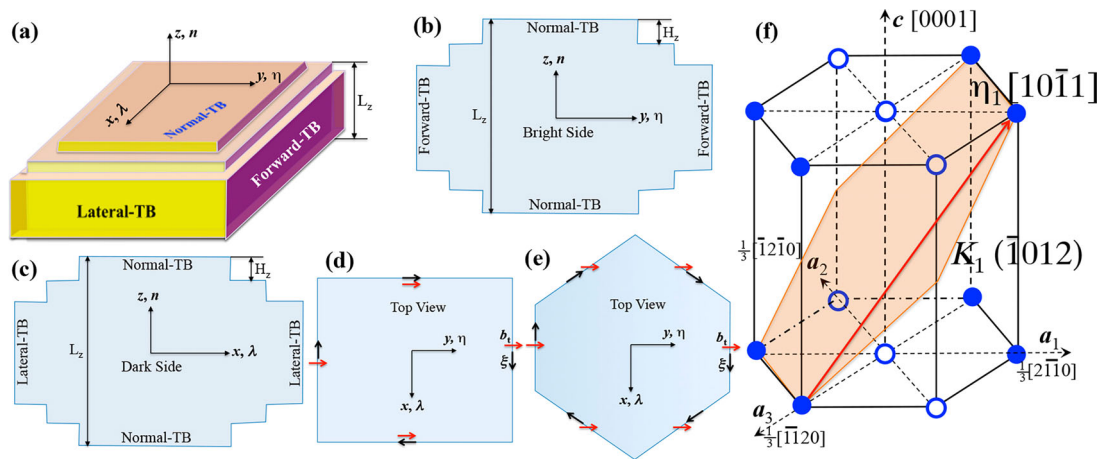
Figure 1. (a) A 3-D ‘cube’ view of a twin domain with x \parallel \lambda , y \parallel \eta , and z \parallel n ; and the thickness L_z . (b) A BS view of the twin with steps that are normal to \eta and have step height H_z . (c) A DS view of the twin with steps that are normal to \lambda and have step height H_z . (d) and (e) A top view of the twin showing a rectangular shape (d) or a hexagonal shape (e). The red arrows indicate the Burgers vector of twinning dislocations, and the black arrows indicate the line sense of twinning dislocations. (f) Coordinates for hcp structure.
