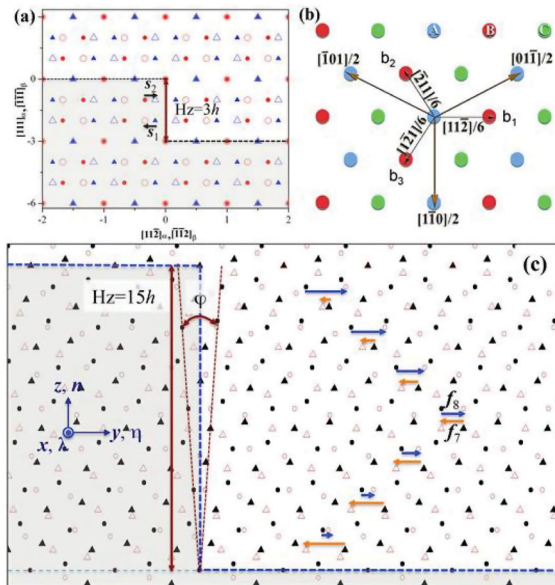
Figure 4. (a) CDP for \Sigma 3(111) twin showing a 3-layer step and the shuffle vectors \mathbf{s}_1 and \mathbf{s}_2 . (b) Plan view of (111) plane stacking and three partials \mathbf{b}_1 , \mathbf{b}_2 , \mathbf{b}_3 . (c) CDC for a (1012) twin viewed in the -\lambda = [\bar{1}2\bar{1}0] direction. Unlike (a), the unit cells of the matrix and twin are relatively rotated by the angle 93.71 degrees about \lambda , creating a disclination (misorientation) angle \varphi of 3.71 degrees. \xi points toward the reader.
